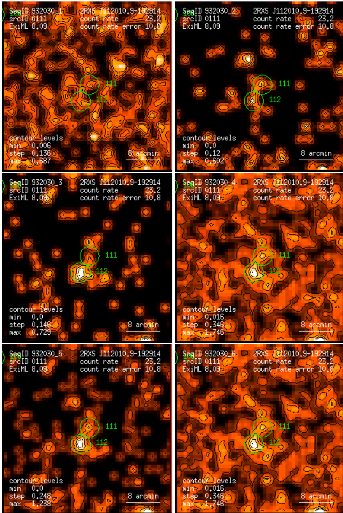
Figure 111: RASS 932030: detection 0111: band rate images, Gaussian filter: (1) PSPC channels 11 – 41, (2) 52 – 90, (3) 91 – 201, (4) 11 – 235, (5) 52 – 201, (6) 11 – 201. Broad band rates in counts/ks. Band rate contour levels in counts/ks/arcmin 2 .
