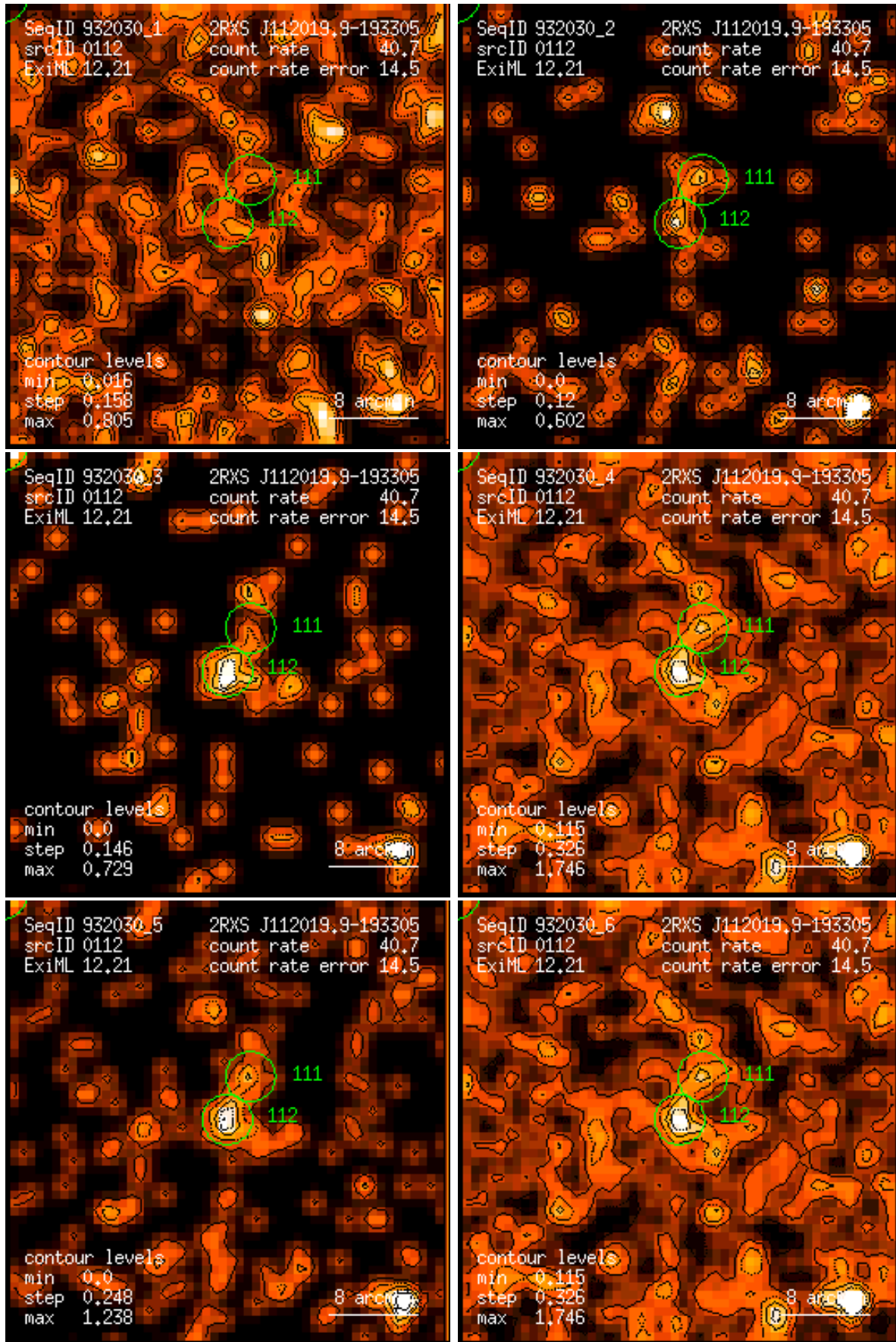
Figure 112: RASS 932030: detection 0112: band rate images, Gaussian filter: (1) PSPC channels 11 – 41, (2) 52 – 90, (3) 91 – 201, (4) 11 – 235, (5) 52 – 201, (6) 11 – 201. Broad band rates in counts/ks. Band rate contour levels in counts/ks/arcmin 2 .
