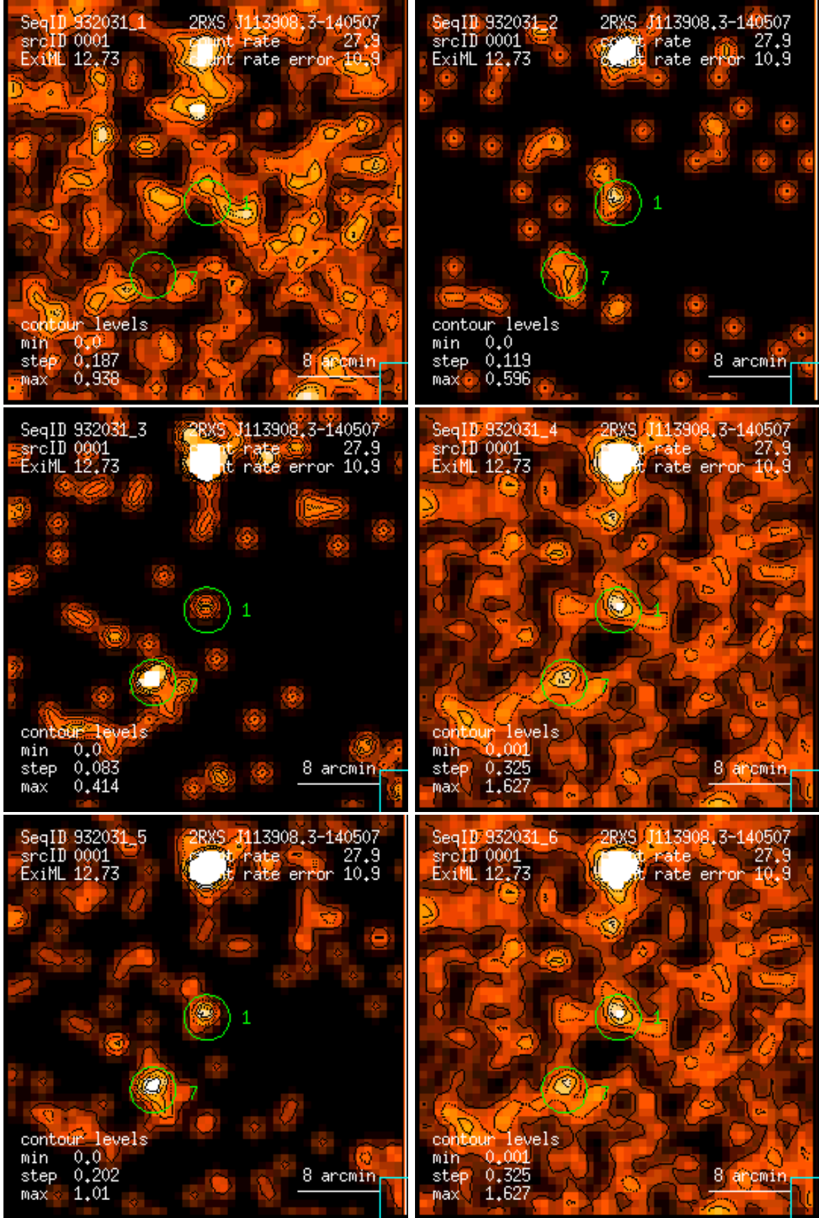
Figure 1: RASS 932031: detection 0001: band rate images, Gaussian filter: (1) PSPC channels 11 – 41, (2) 52 – 90, (3) 91 – 201, (4) 11 – 235, (5) 52 – 201, (6) 11 – 201. Broad band rates in counts/ks. Band rate contour levels in counts/ks/arcmin 2 .
