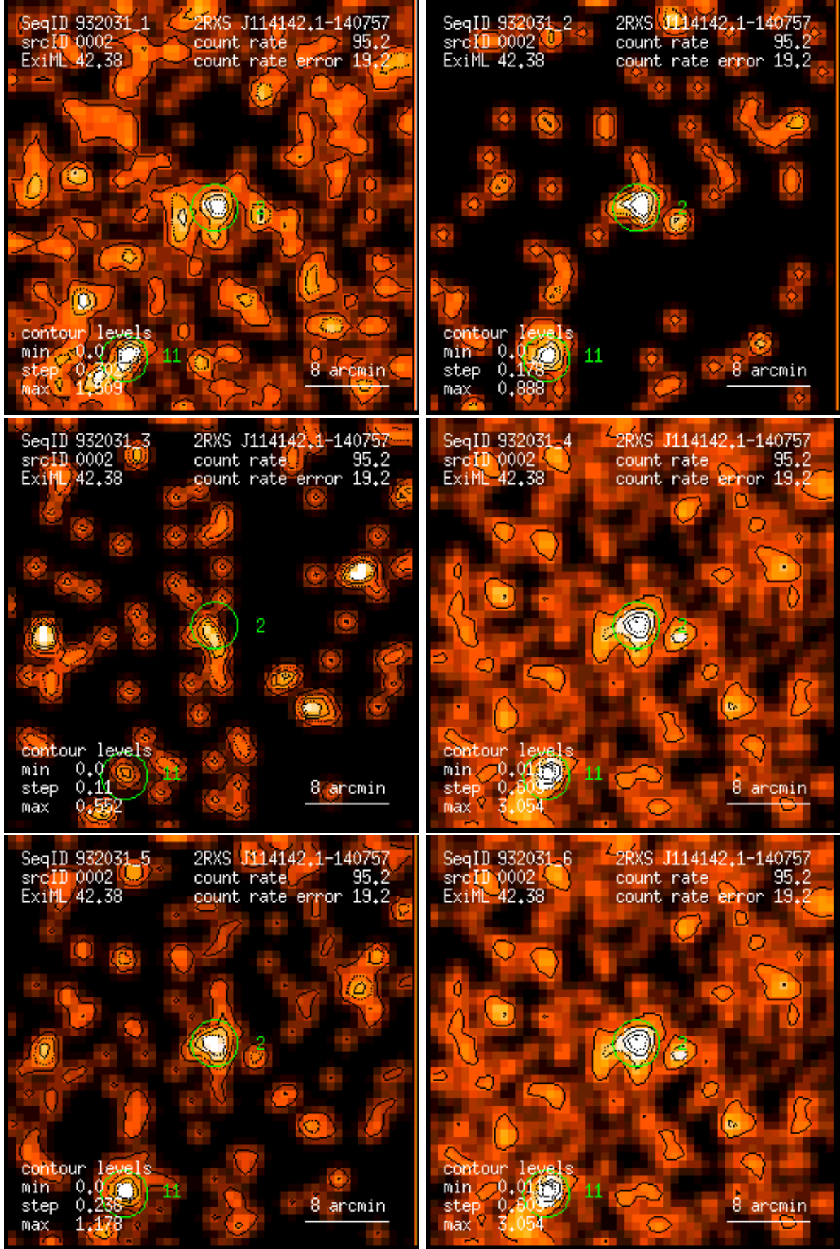
Figure 2: RASS 932031: detection 0002: band rate images, Gaussian filter: (1) PSPC channels 11 – 41, (2) 52 – 90, (3) 91 – 201, (4) 11 – 235, (5) 52 – 201, (6) 11 – 201. Broad band rates in counts/ks. Band rate contour levels in counts/ks/arcmin 2 .
