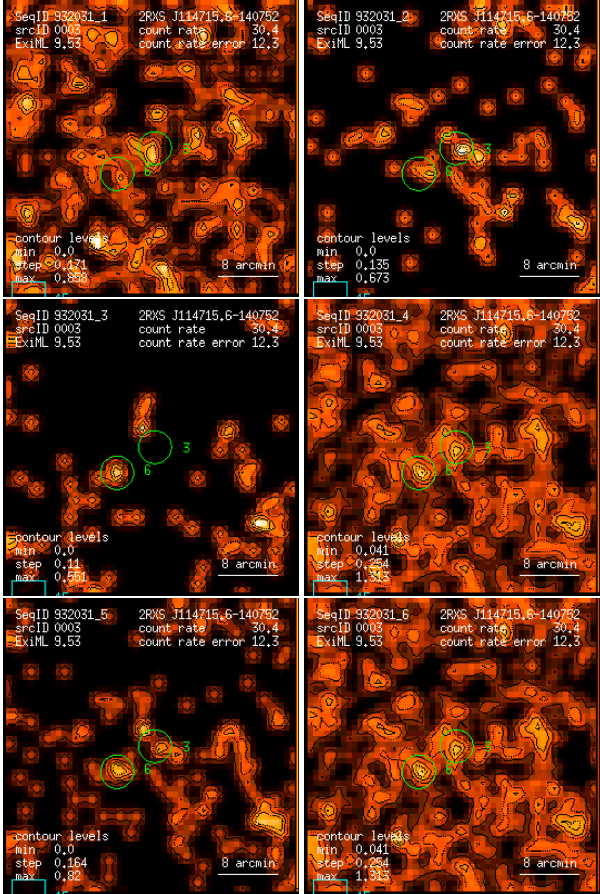
Figure 3: RASS 932031: detection 0003: band rate images, Gaussian filter: (1) PSPC channels 11 – 41, (2) 52 – 90, (3) 91 – 201, (4) 11 – 235, (5) 52 – 201, (6) 11 – 201. Broad band rates in counts/ks. Band rate contour levels in counts/ks/arcmin 2 .
