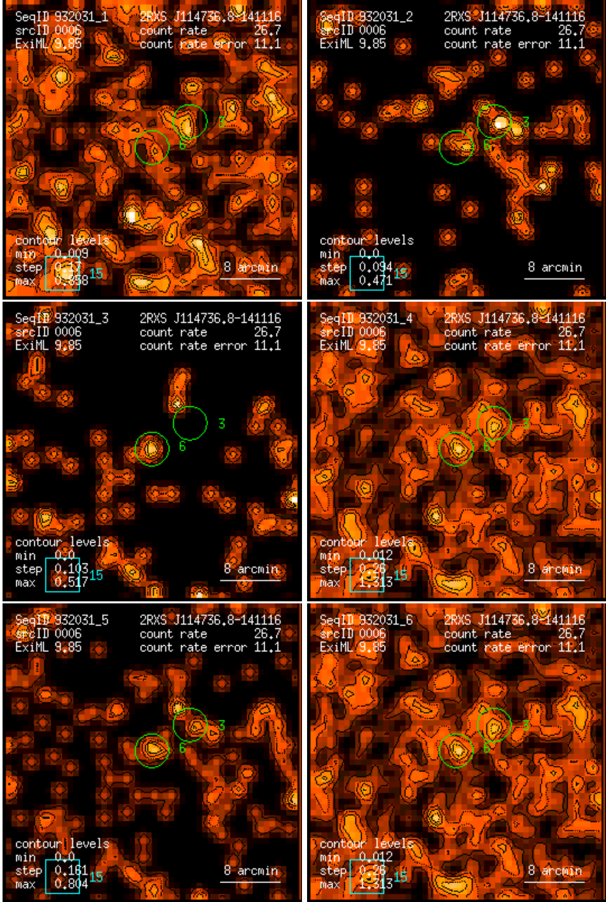
Figure 6: RASS 932031: detection 0006: band rate images, Gaussian filter: (1) PSPC channels 11 – 41, (2) 52 – 90, (3) 91 – 201, (4) 11 – 235, (5) 52 – 201, (6) 11 – 201. Broad band rates in counts/ks. Band rate contour levels in counts/ks/arcmin 2 .
