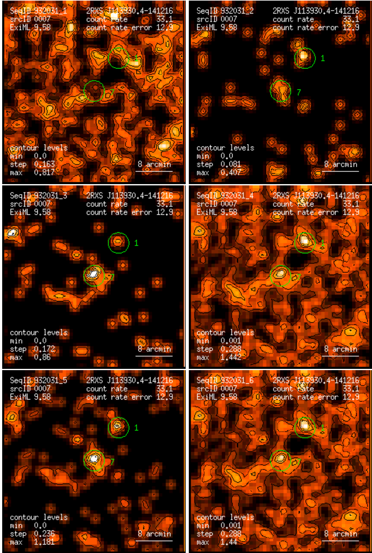
Figure 7: RASS 932031: detection 0007: band rate images, Gaussian filter: (1) PSPC channels 11 – 41, (2) 52 – 90, (3) 91 – 201, (4) 11 – 235, (5) 52 – 201, (6) 11 – 201. Broad band rates in counts/ks. Band rate contour levels in counts/ks/arcmin 2 .
