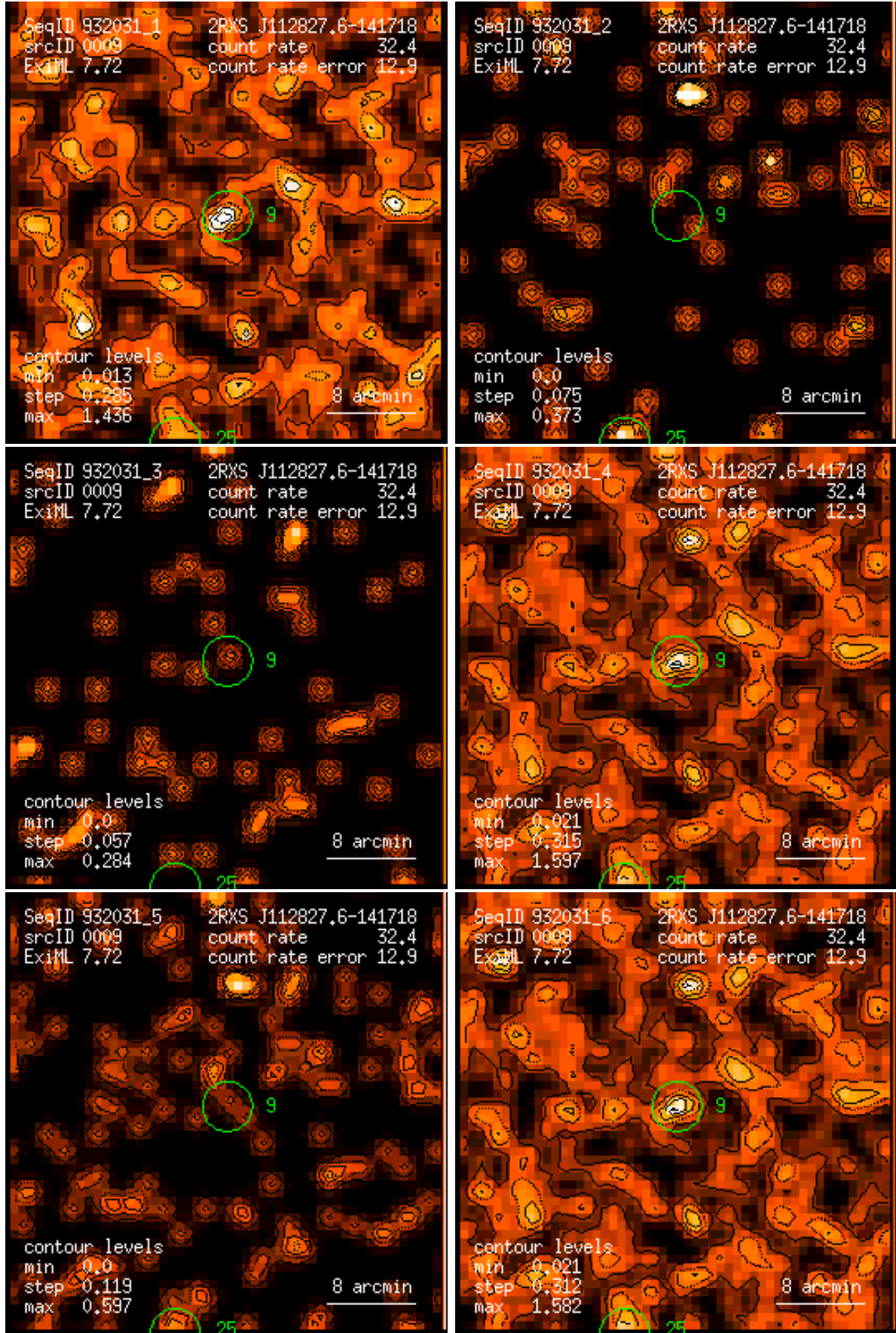
Figure 9: RASS 932031: detection 0009: band rate images, Gaussian filter: (1) PSPC channels 11 – 41, (2) 52 – 90, (3) 91 – 201, (4) 11 – 235, (5) 52 – 201, (6) 11 – 201. Broad band rates in counts/ks. Band rate contour levels in counts/ks/arcmin 2 .
