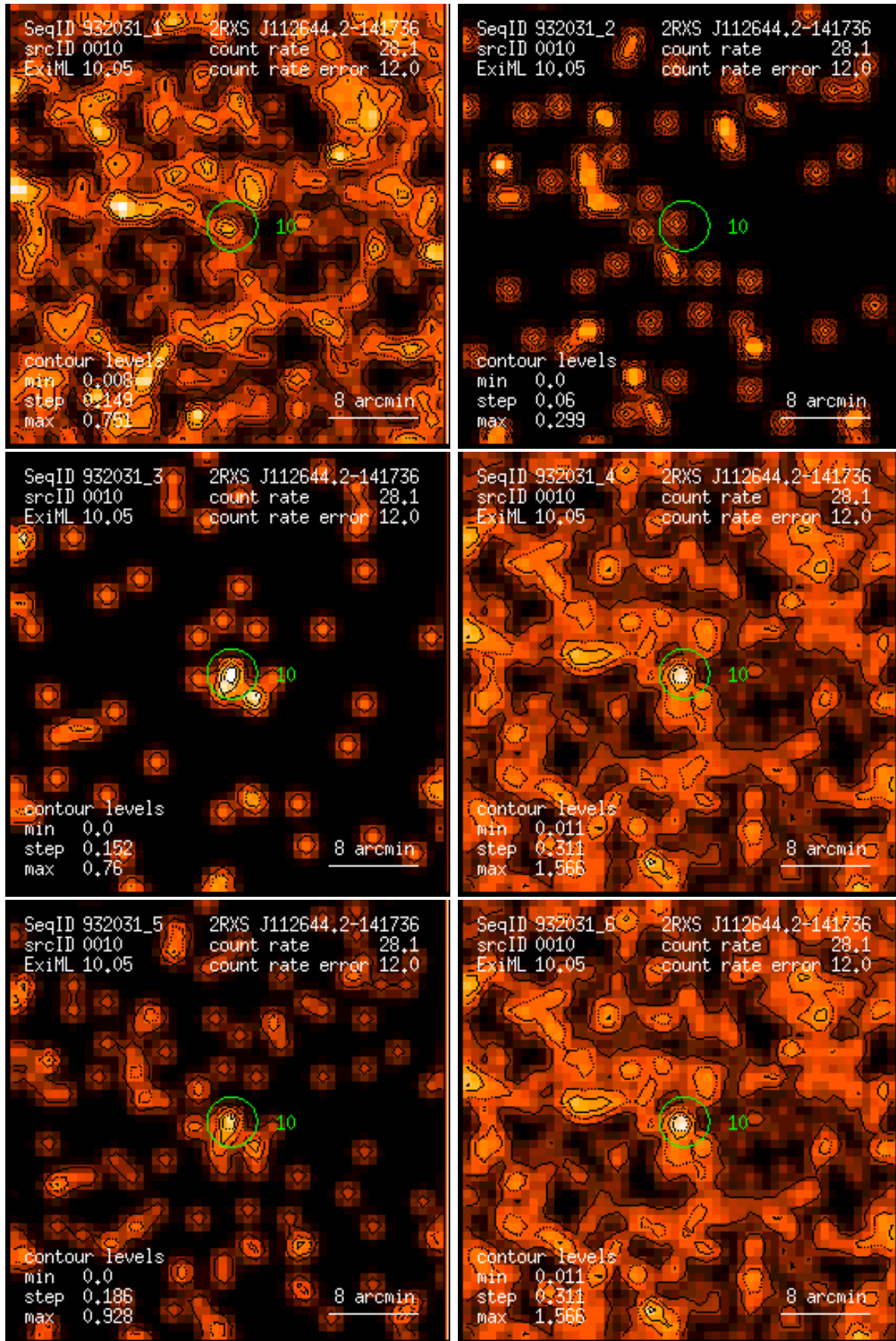
Figure 10: RASS 932031: detection 0010: band rate images, Gaussian filter: (1) PSPC channels 11 – 41, (2) 52 – 90, (3) 91 – 201, (4) 11 – 235, (5) 52 – 201, (6) 11 – 201. Broad band rates in counts/ks. Band rate contour levels in counts/ks/arcmin 2 .
