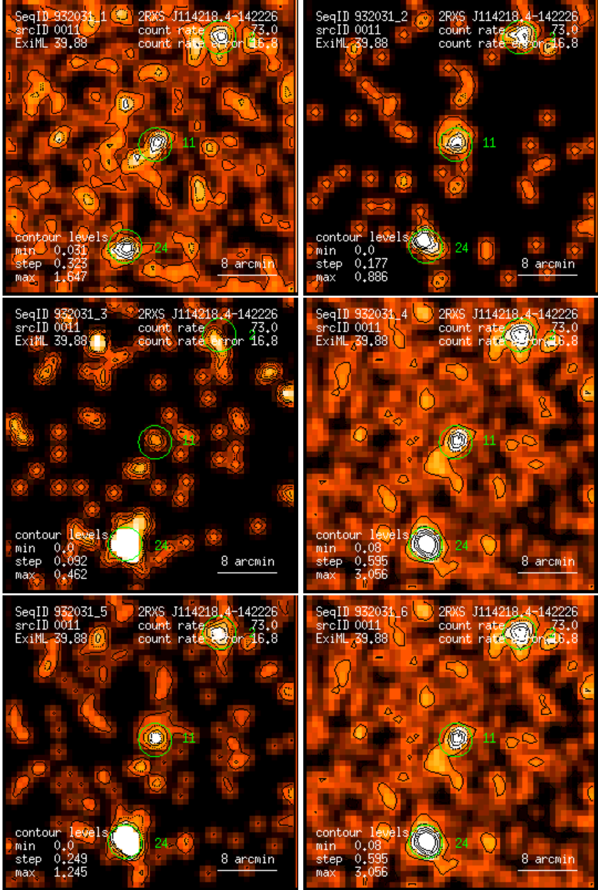
Figure 11: RASS 932031: detection 0011: band rate images, Gaussian filter: (1) PSPC channels 11 – 41, (2) 52 – 90, (3) 91 – 201, (4) 11 – 235, (5) 52 – 201, (6) 11 – 201. Broad band rates in counts/ks. Band rate contour levels in counts/ks/arcmin 2 .
