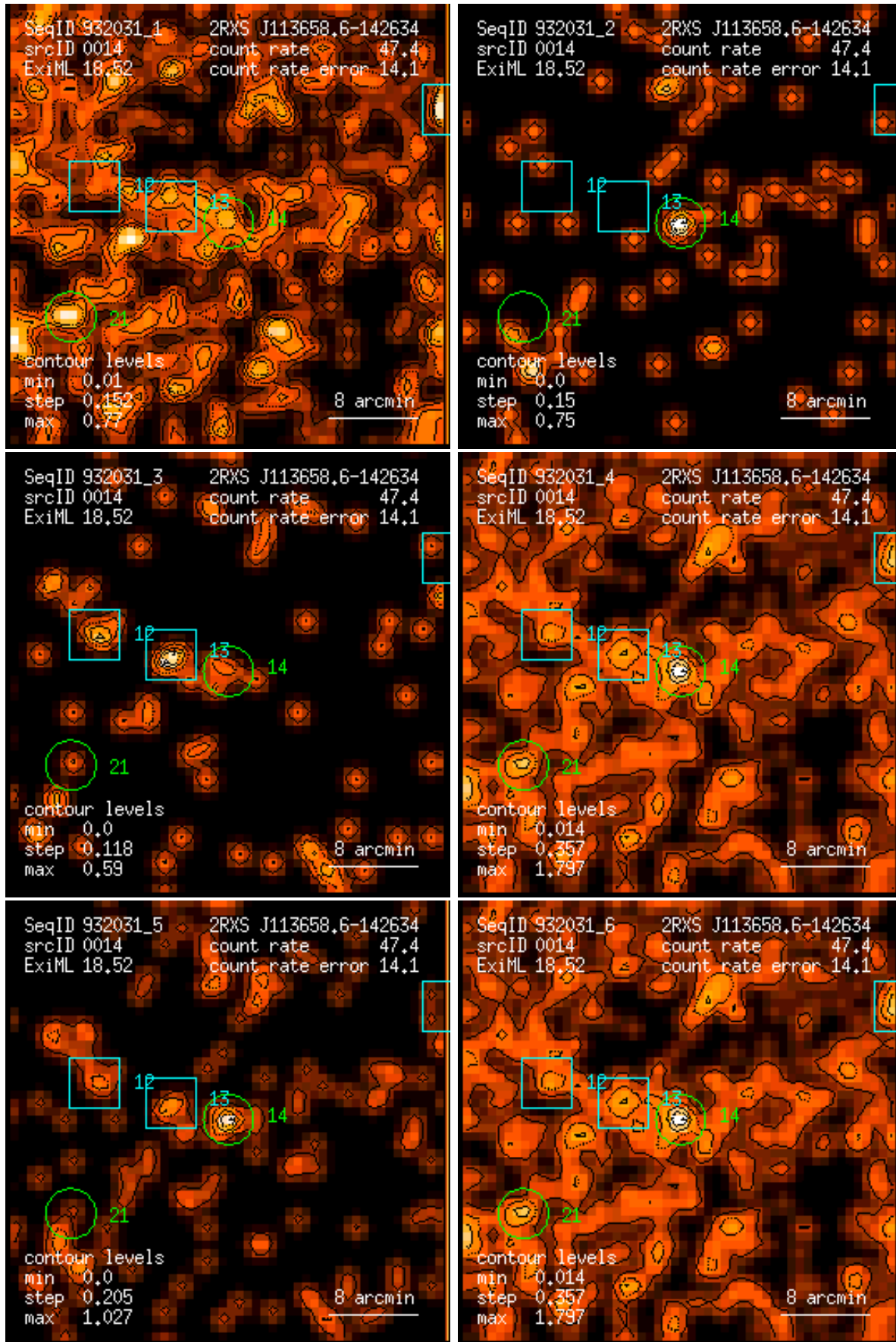
Figure 14: RASS 932031: detection 0014: band rate images, Gaussian filter: (1) PSPC channels 11 – 41, (2) 52 – 90, (3) 91 – 201, (4) 11 – 235, (5) 52 – 201, (6) 11 – 201. Broad band rates in counts/ks. Band rate contour levels in counts/ks/arcmin 2 .
