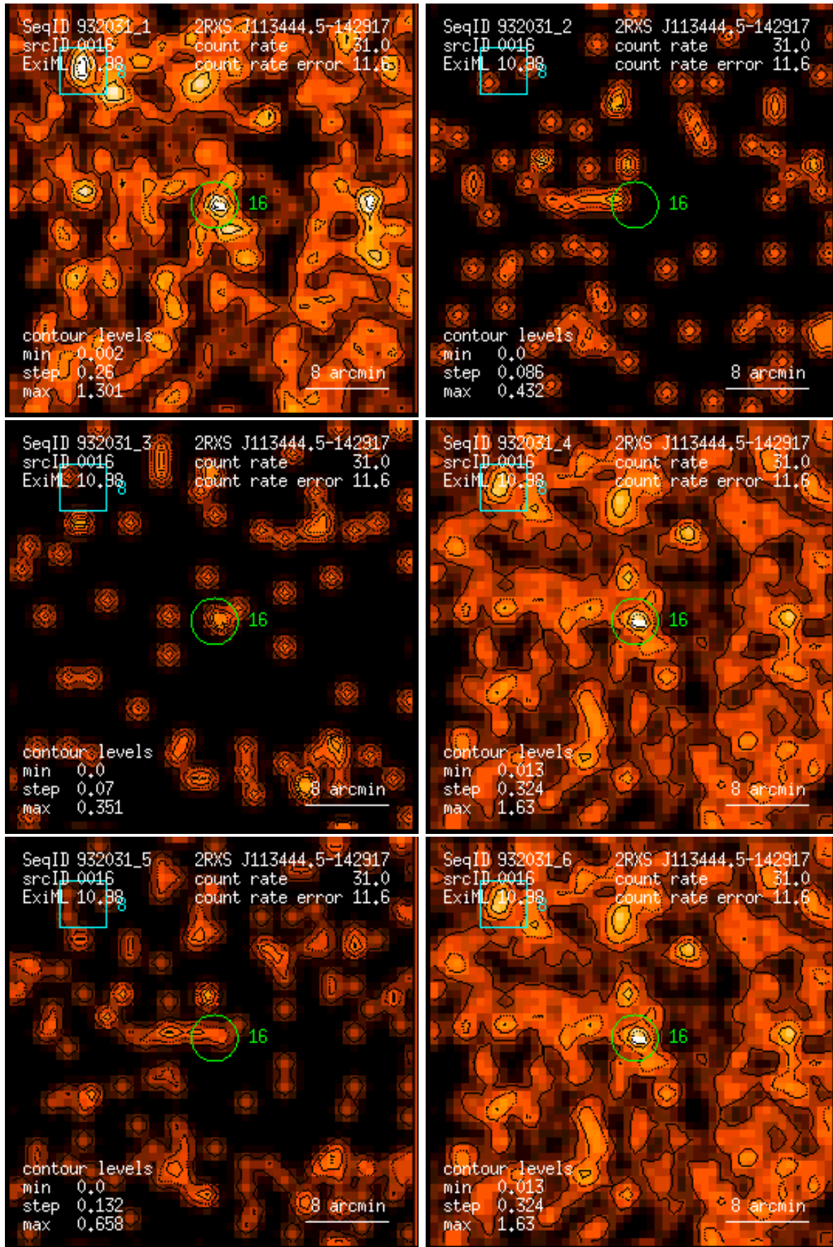
Figure 16: RASS 932031: detection 0016: band rate images, Gaussian filter: (1) PSPC channels 11 – 41, (2) 52 – 90, (3) 91 – 201, (4) 11 – 235, (5) 52 – 201, (6) 11 – 201. Broad band rates in counts/ks. Band rate contour levels in counts/ks/arcmin 2 .
