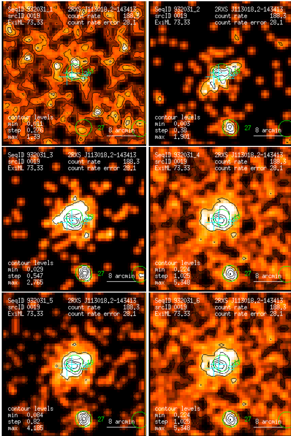
Figure 19: RASS 932031: detection 0019: band rate images, Gaussian filter: (1) PSPC channels 11 – 41, (2) 52 – 90, (3) 91 – 201, (4) 11 – 235, (5) 52 – 201, (6) 11 – 201. Broad band rates in counts/ks. Band rate contour levels in counts/ks/arcmin 2 .
