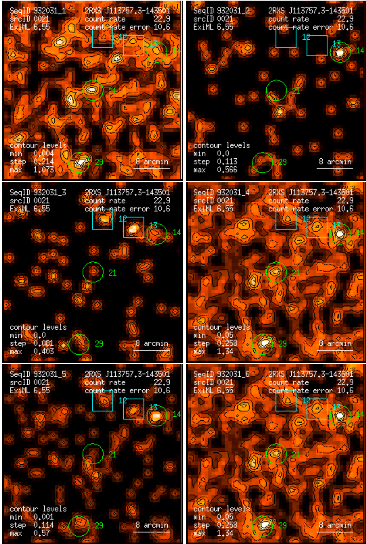
Figure 21: RASS 932031: detection 0021: band rate images, Gaussian filter: (1) PSPC channels 11 – 41, (2) 52 – 90, (3) 91 – 201, (4) 11 – 235, (5) 52 – 201, (6) 11 – 201. Broad band rates in counts/ks. Band rate contour levels in counts/ks/arcmin 2 .
