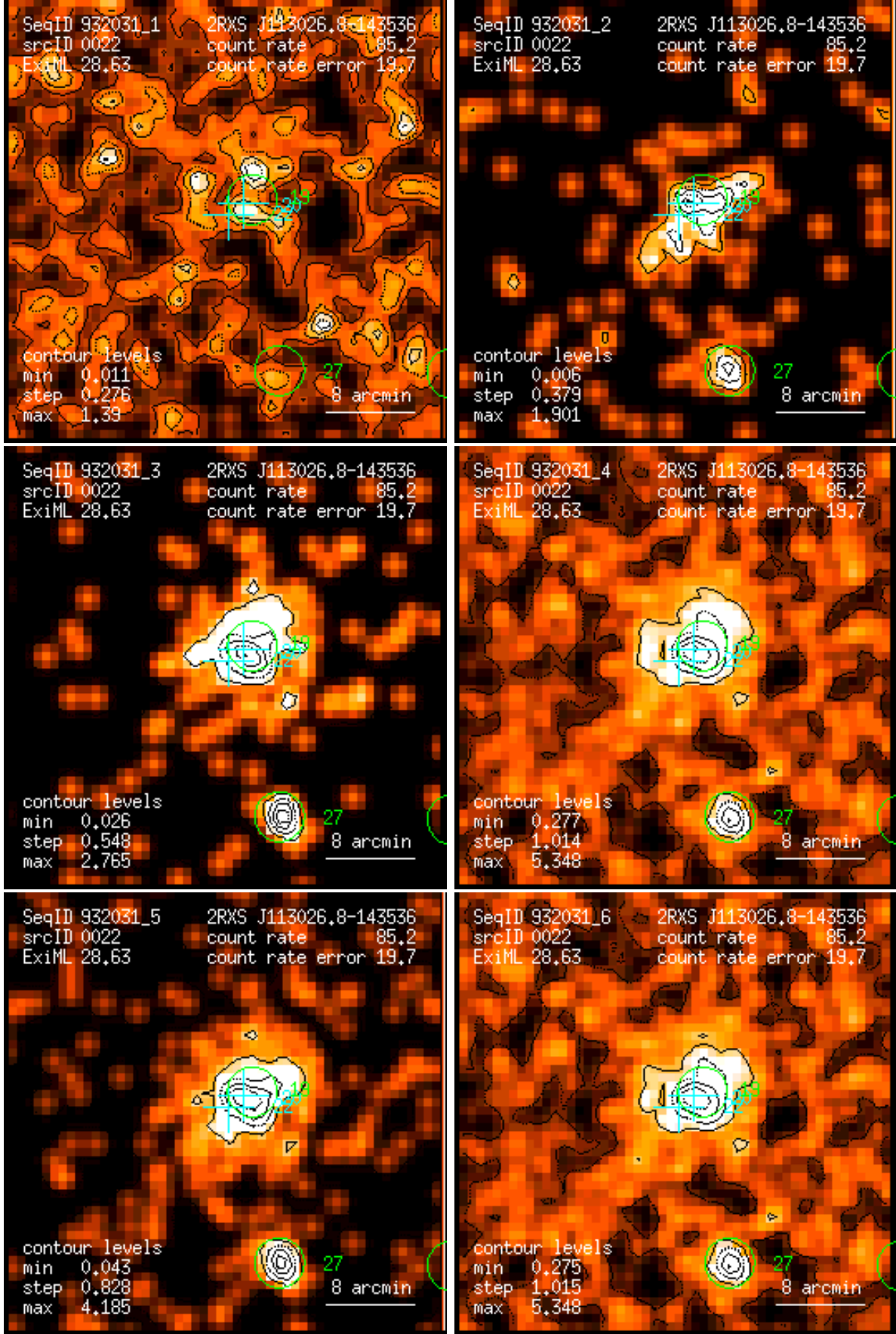
Figure 22: RASS 932031: detection 0022: band rate images, Gaussian filter: (1) PSPC channels 11 – 41, (2) 52 – 90, (3) 91 – 201, (4) 11 – 235, (5) 52 – 201, (6) 11 – 201. Broad band rates in counts/ks. Band rate contour levels in counts/ks/arcmin 2 .
