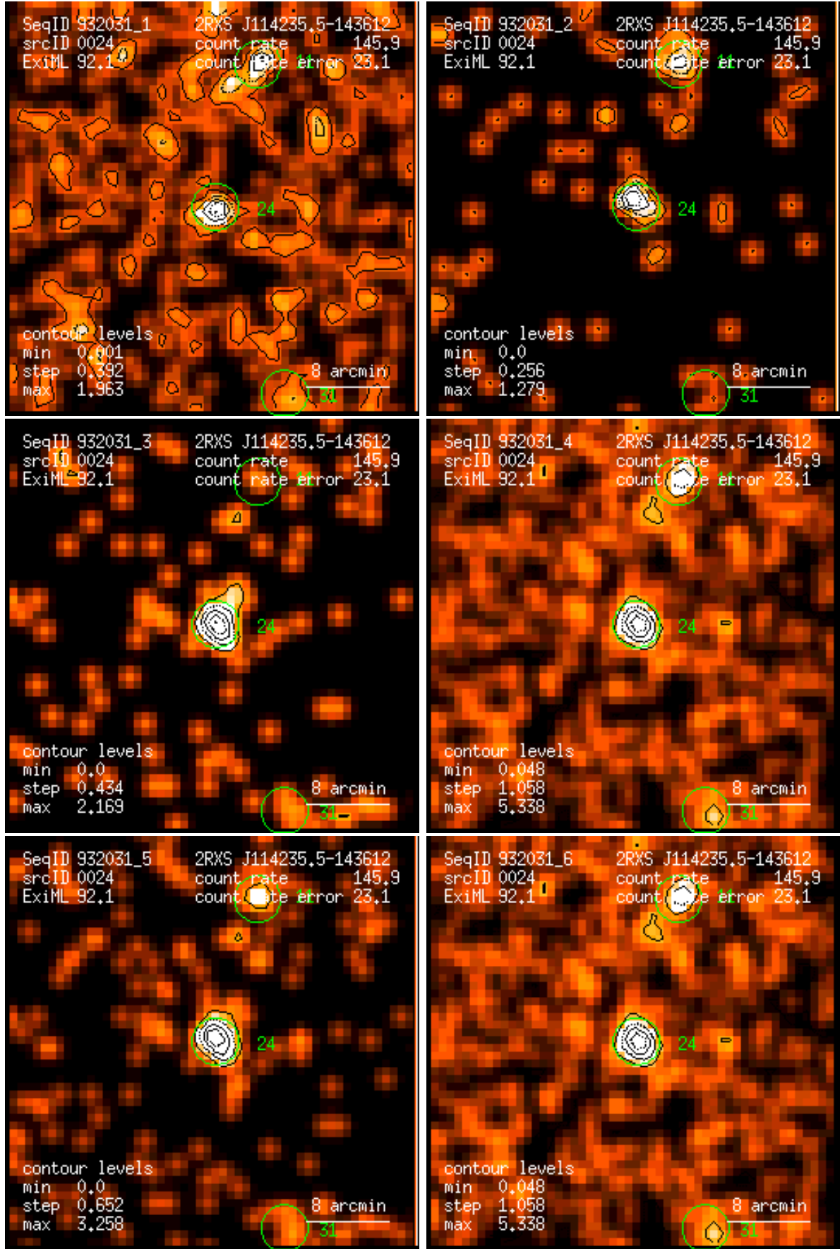
Figure 24: RASS 932031: detection 0024: band rate images, Gaussian filter: (1) PSPC channels 11 – 41, (2) 52 – 90, (3) 91 – 201, (4) 11 – 235, (5) 52 – 201, (6) 11 – 201. Broad band rates in counts/ks. Band rate contour levels in counts/ks/arcmin 2 .
