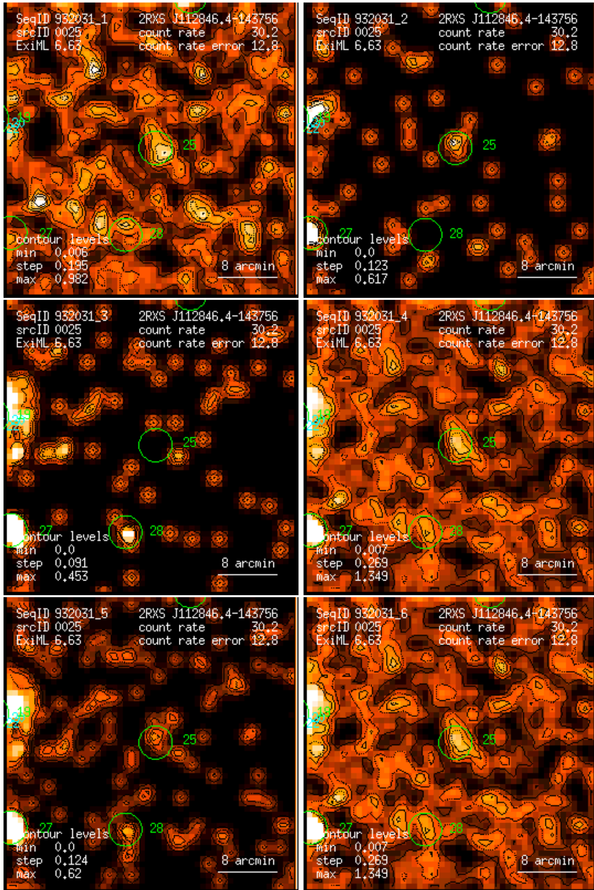
Figure 25: RASS 932031: detection 0025: band rate images, Gaussian filter: (1) PSPC channels 11 – 41, (2) 52 – 90, (3) 91 – 201, (4) 11 – 235, (5) 52 – 201, (6) 11 – 201. Broad band rates in counts/ks. Band rate contour levels in counts/ks/arcmin 2 .
