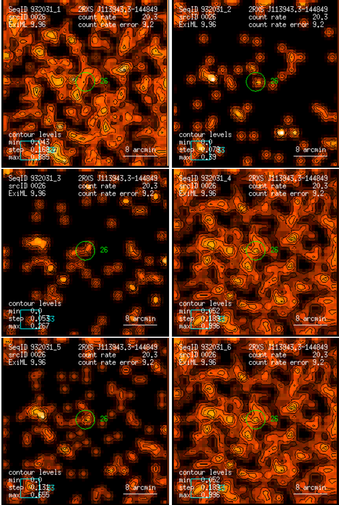
Figure 26: RASS 932031: detection 0026: band rate images, Gaussian filter: (1) PSPC channels 11 – 41, (2) 52 – 90, (3) 91 – 201, (4) 11 – 235, (5) 52 – 201, (6) 11 – 201. Broad band rates in counts/ks. Band rate contour levels in counts/ks/arcmin 2 .
