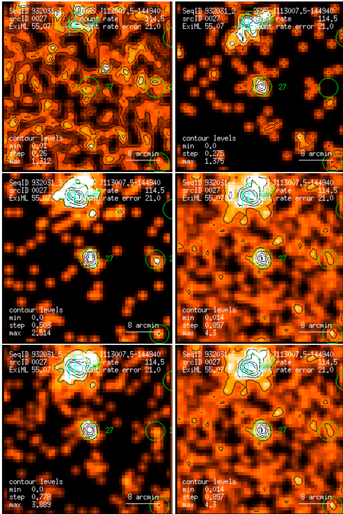
Figure 27: RASS 932031: detection 0027: band rate images, Gaussian filter: (1) PSPC channels 11 – 41, (2) 52 – 90, (3) 91 – 201, (4) 11 – 235, (5) 52 – 201, (6) 11 – 201. Broad band rates in counts/ks. Band rate contour levels in counts/ks/arcmin 2 .
