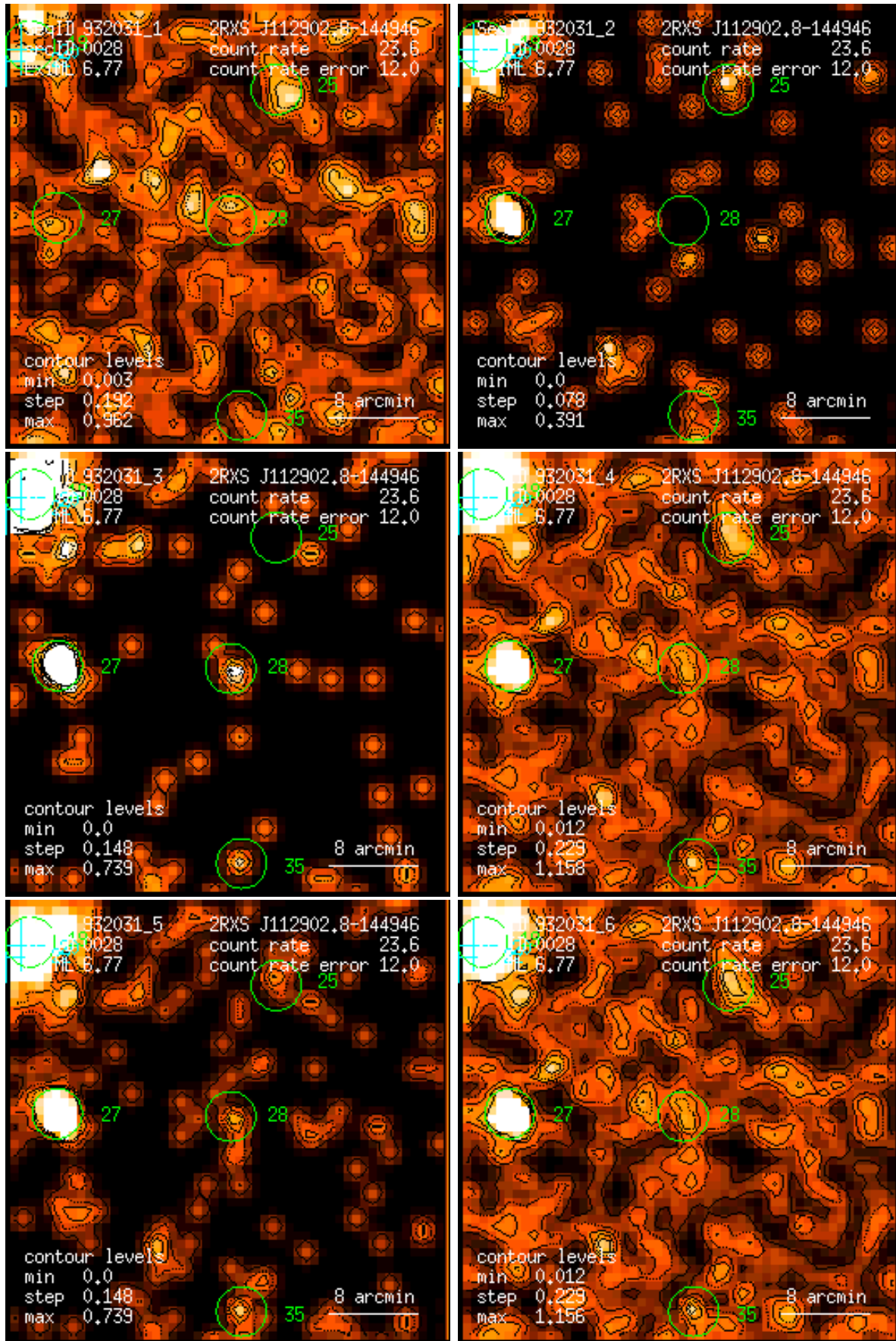
Figure 28: RASS 932031: detection 0028: band rate images, Gaussian filter: (1) PSPC channels 11 – 41, (2) 52 – 90, (3) 91 – 201, (4) 11 – 235, (5) 52 – 201, (6) 11 – 201. Broad band rates in counts/ks. Band rate contour levels in counts/ks/arcmin 2 .
