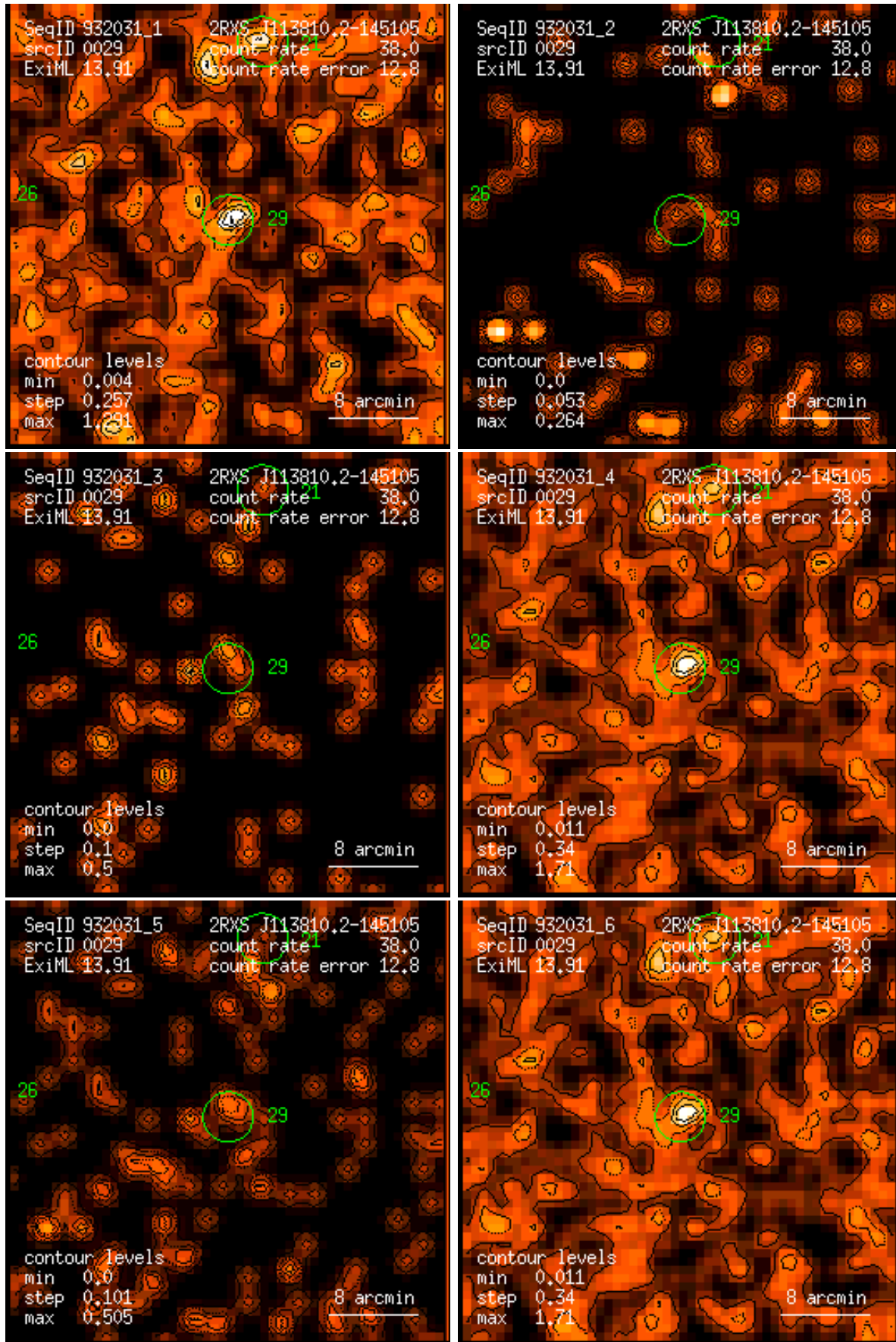
Figure 29: RASS 932031: detection 0029: band rate images, Gaussian filter: (1) PSPC channels 11 – 41, (2) 52 – 90, (3) 91 – 201, (4) 11 – 235, (5) 52 – 201, (6) 11 – 201. Broad band rates in counts/ks. Band rate contour levels in counts/ks/arcmin 2 .
