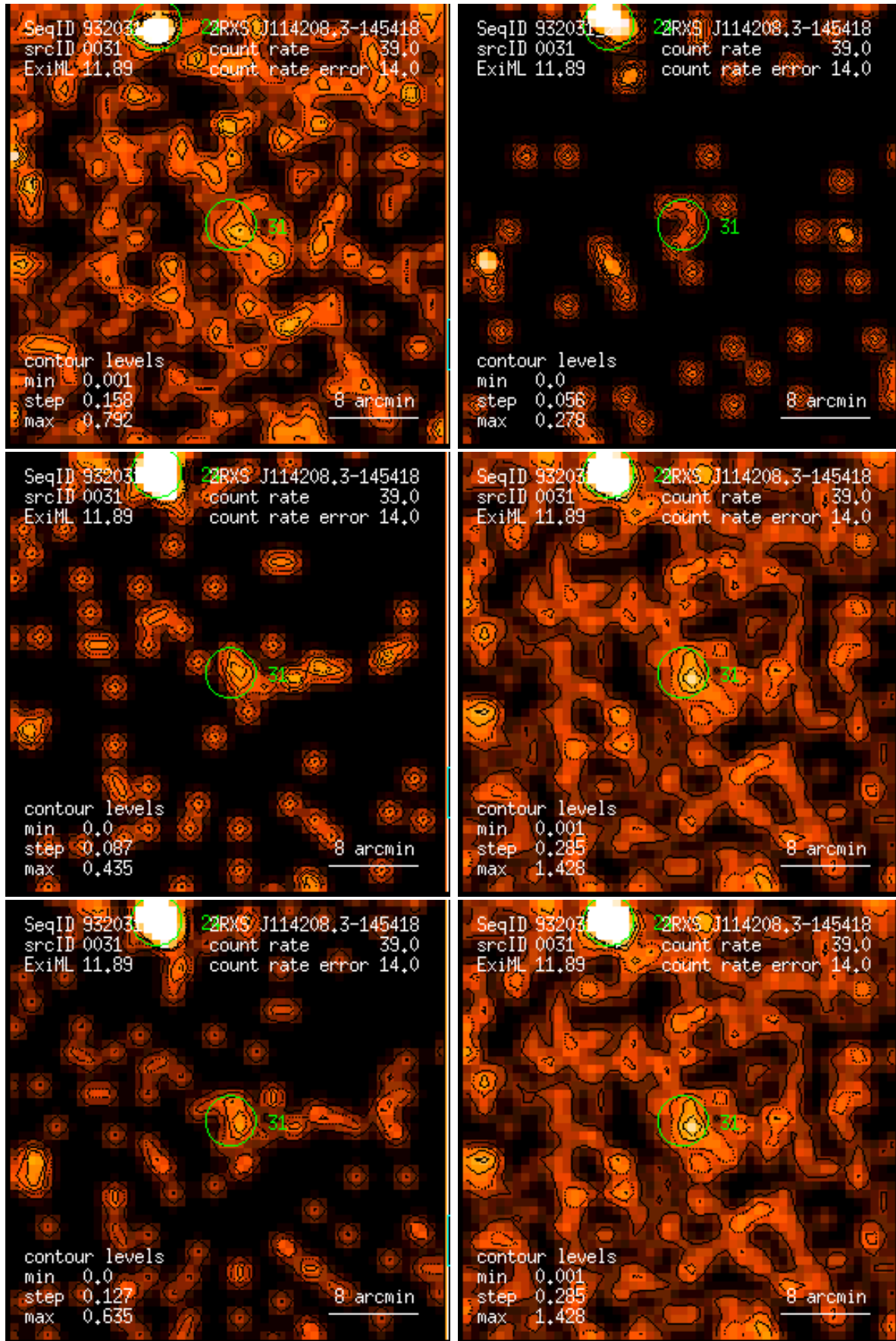
Figure 31: RASS 932031: detection 0031: band rate images, Gaussian filter: (1) PSPC channels 11 – 41, (2) 52 – 90, (3) 91 – 201, (4) 11 – 235, (5) 52 – 201, (6) 11 – 201. Broad band rates in counts/ks. Band rate contour levels in counts/ks/arcmin 2 .
