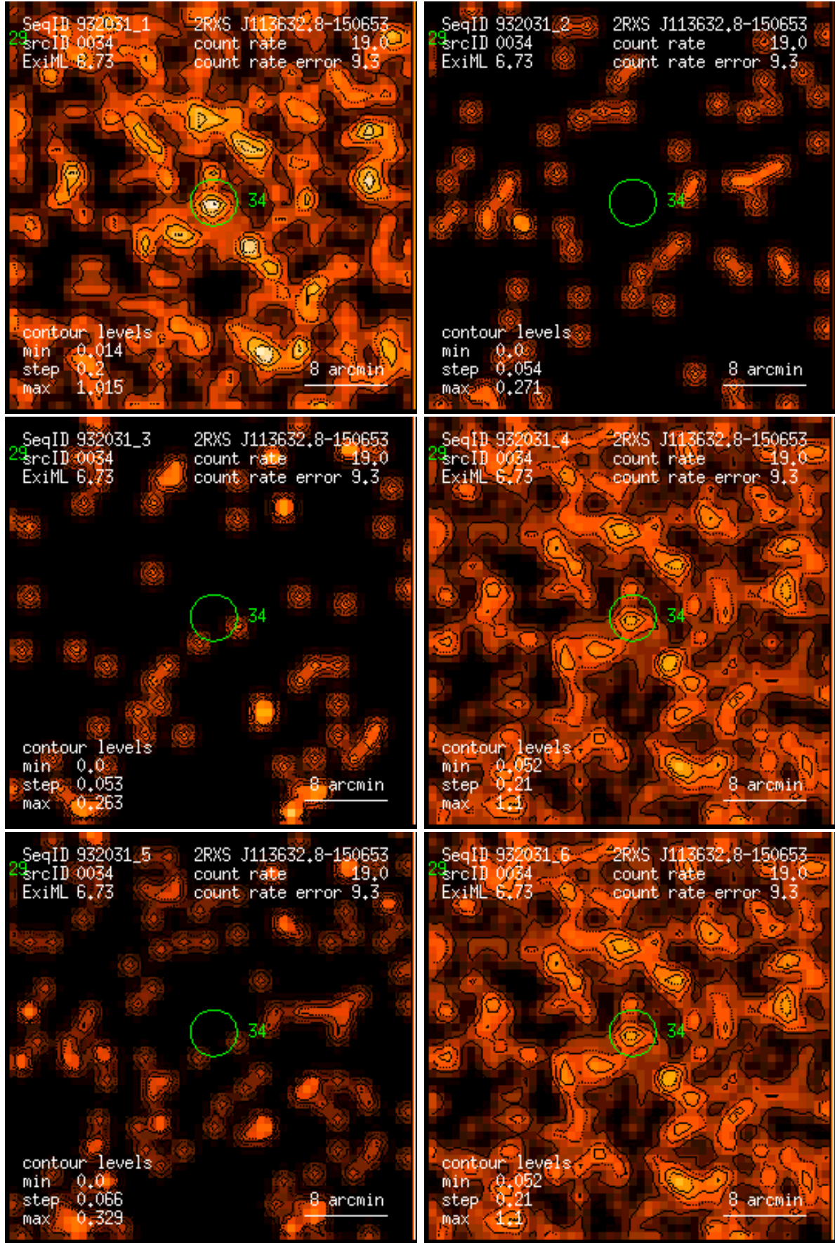
Figure 34: RASS 932031: detection 0034: band rate images, Gaussian filter: (1) PSPC channels 11 – 41, (2) 52 – 90, (3) 91 – 201, (4) 11 – 235, (5) 52 – 201, (6) 11 – 201. Broad band rates in counts/ks. Band rate contour levels in counts/ks/arcmin 2 .
