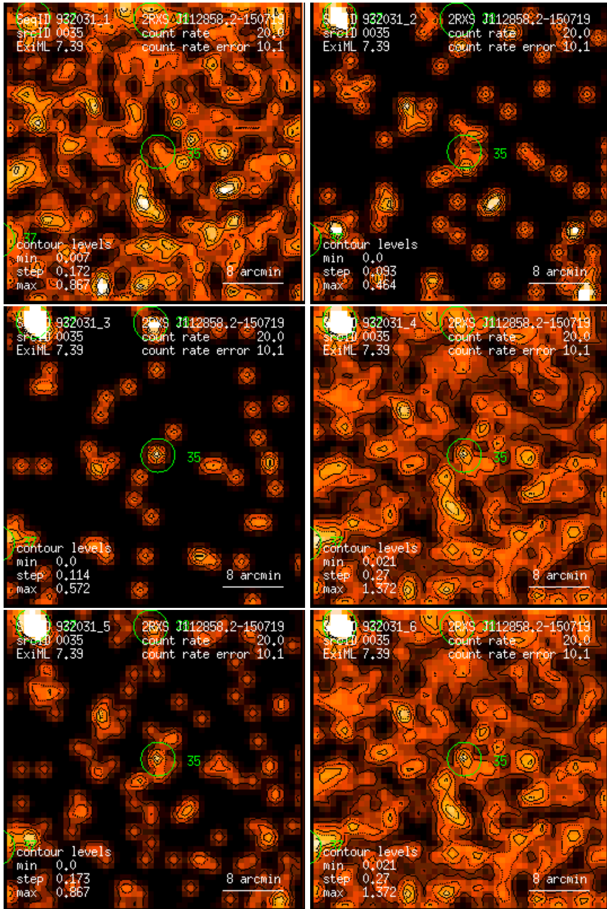
Figure 35: RASS 932031: detection 0035: band rate images, Gaussian filter: (1) PSPC channels 11 – 41, (2) 52 – 90, (3) 91 – 201, (4) 11 – 235, (5) 52 – 201, (6) 11 – 201. Broad band rates in counts/ks. Band rate contour levels in counts/ks/arcmin 2 .
