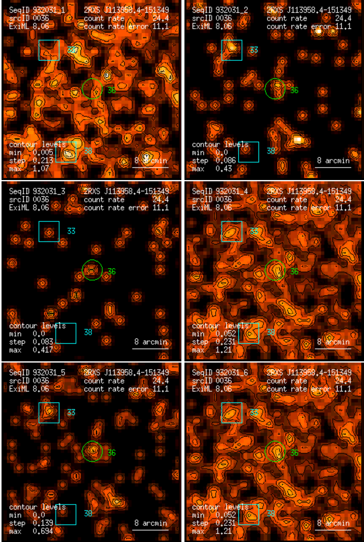
Figure 36: RASS 932031: detection 0036: band rate images, Gaussian filter: (1) PSPC channels 11 – 41, (2) 52 – 90, (3) 91 – 201, (4) 11 – 235, (5) 52 – 201, (6) 11 – 201. Broad band rates in counts/ks. Band rate contour levels in counts/ks/arcmin 2 .
