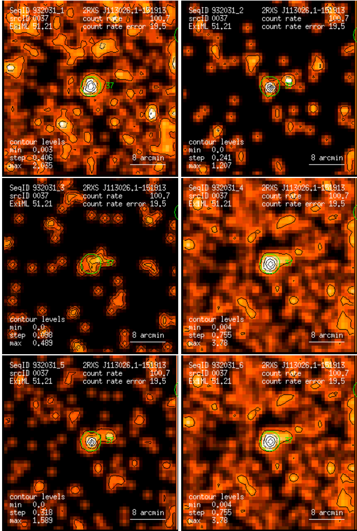
Figure 37: RASS 932031: detection 0037: band rate images, Gaussian filter: (1) PSPC channels 11 – 41, (2) 52 – 90, (3) 91 – 201, (4) 11 – 235, (5) 52 – 201, (6) 11 – 201. Broad band rates in counts/ks. Band rate contour levels in counts/ks/arcmin 2 .
