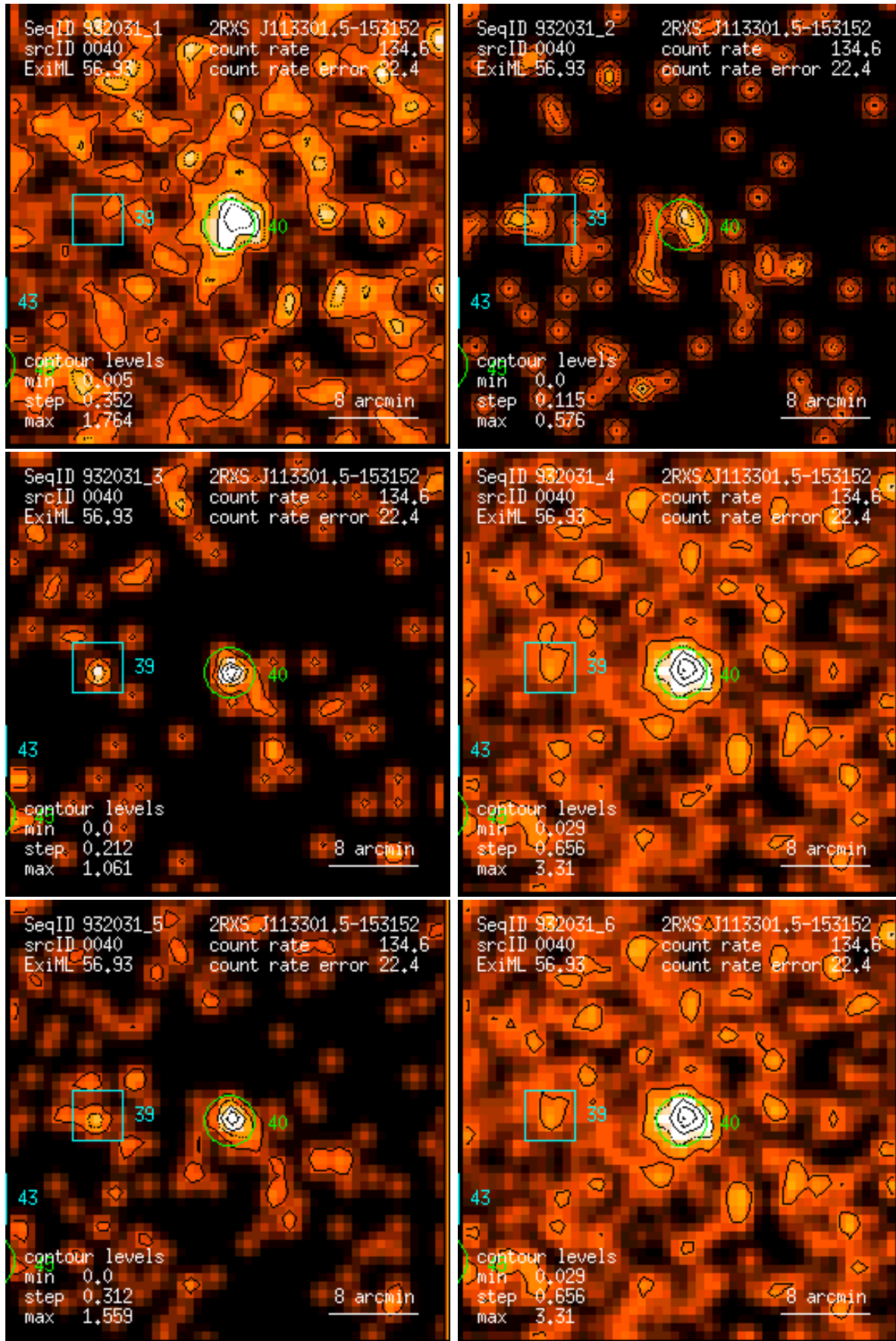
Figure 40: RASS 932031: detection 0040: band rate images, Gaussian filter: (1) PSPC channels 11 – 41, (2) 52 – 90, (3) 91 – 201, (4) 11 – 235, (5) 52 – 201, (6) 11 – 201. Broad band rates in counts/ks. Band rate contour levels in counts/ks/arcmin 2 .
