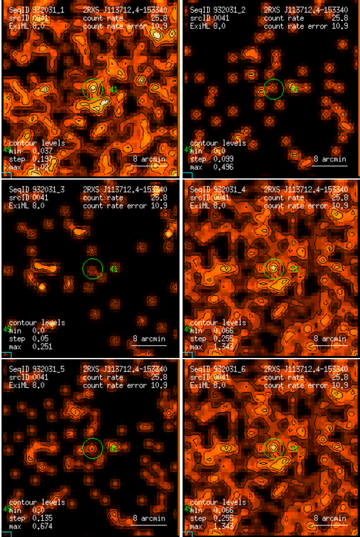
Figure 41: RASS 932031: detection 0041: band rate images, Gaussian filter: (1) PSPC channels 11 – 41, (2) 52 – 90, (3) 91 – 201, (4) 11 – 235, (5) 52 – 201, (6) 11 – 201. Broad band rates in counts/ks. Band rate contour levels in counts/ks/arcmin 2 .
