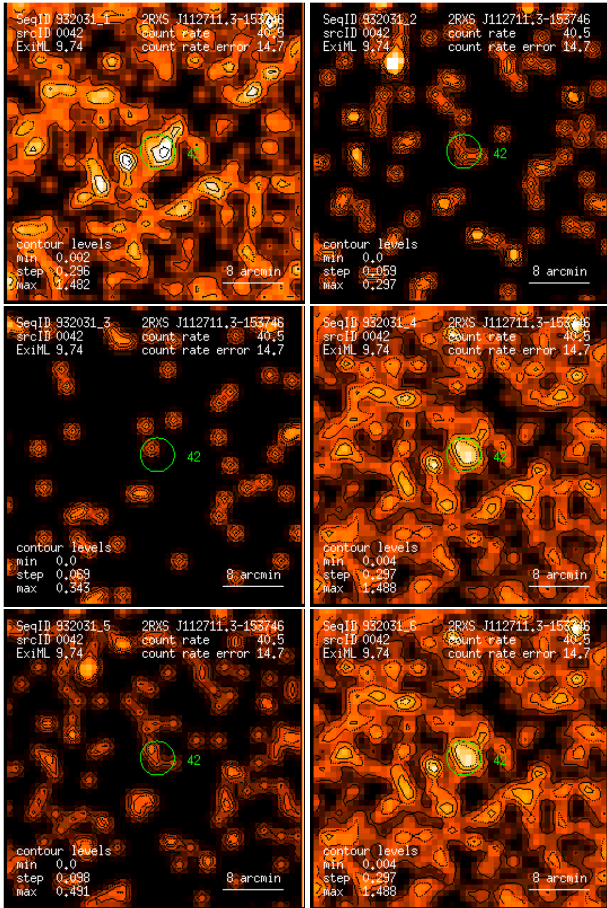
Figure 42: RASS 932031: detection 0042: band rate images, Gaussian filter: (1) PSPC channels 11 – 41, (2) 52 – 90, (3) 91 – 201, (4) 11 – 235, (5) 52 – 201, (6) 11 – 201. Broad band rates in counts/ks. Band rate contour levels in counts/ks/arcmin 2 .
