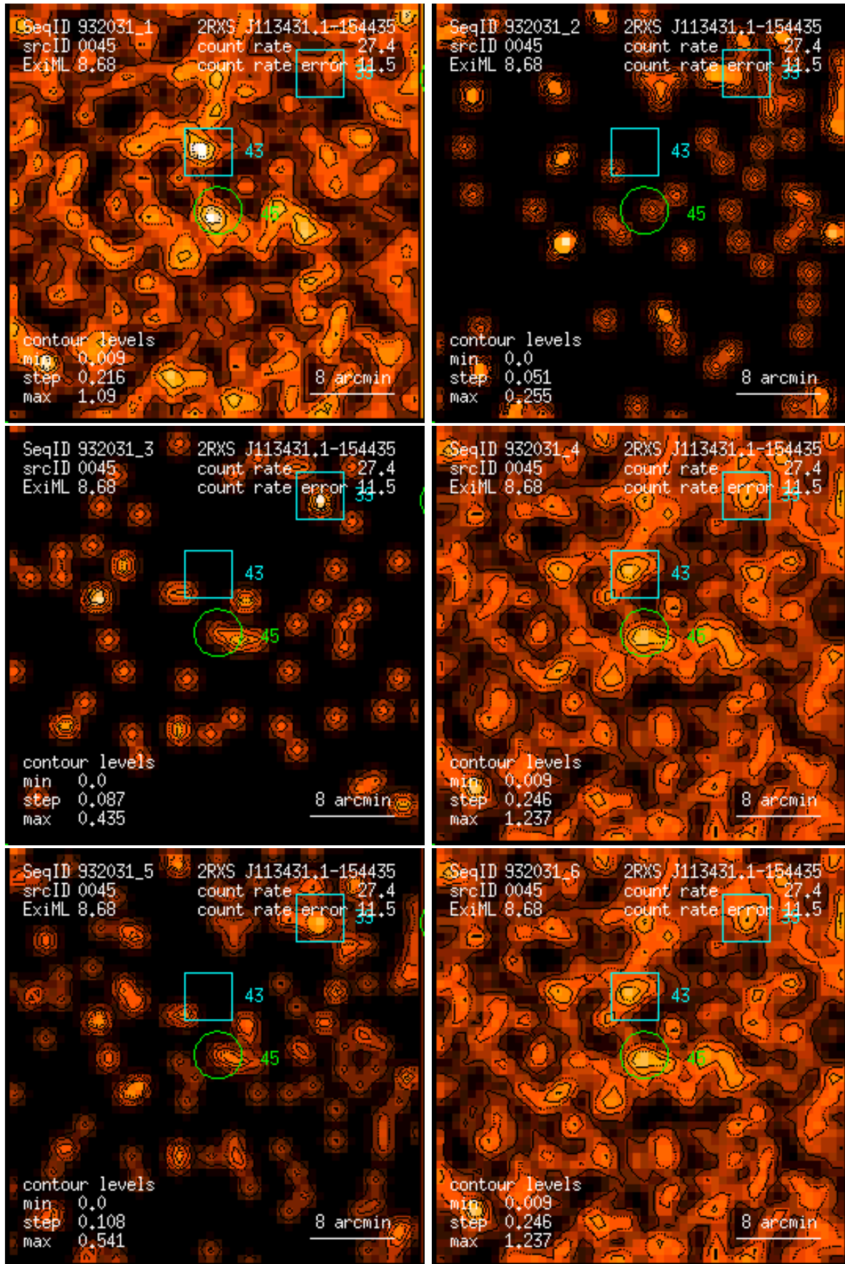
Figure 45: RASS 932031: detection 0045: band rate images, Gaussian filter: (1) PSPC channels 11 – 41, (2) 52 – 90, (3) 91 – 201, (4) 11 – 235, (5) 52 – 201, (6) 11 – 201. Broad band rates in counts/ks. Band rate contour levels in counts/ks/arcmin 2 .
