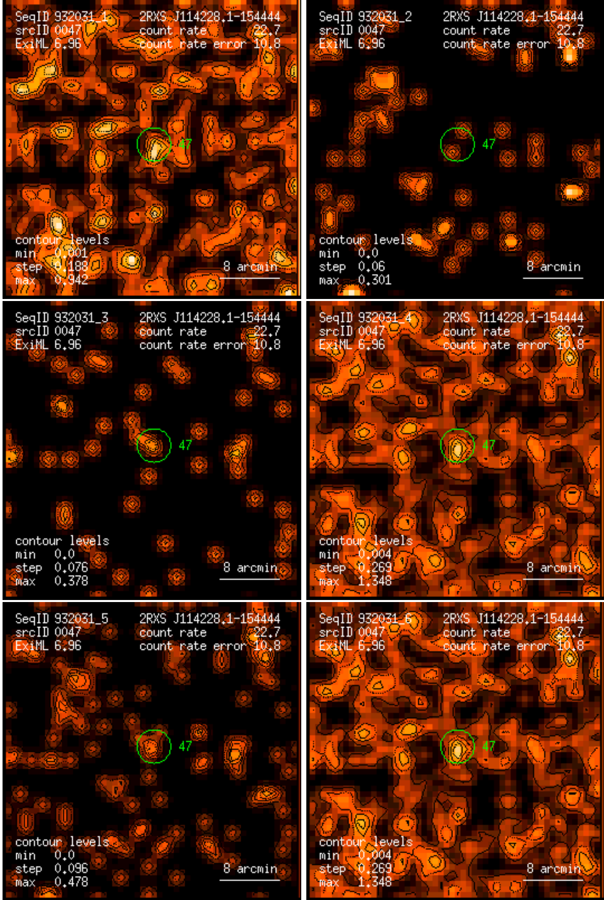
Figure 47: RASS 932031: detection 0047: band rate images, Gaussian filter: (1) PSPC channels 11 – 41, (2) 52 – 90, (3) 91 – 201, (4) 11 – 235, (5) 52 – 201, (6) 11 – 201. Broad band rates in counts/ks. Band rate contour levels in counts/ks/arcmin 2 .
