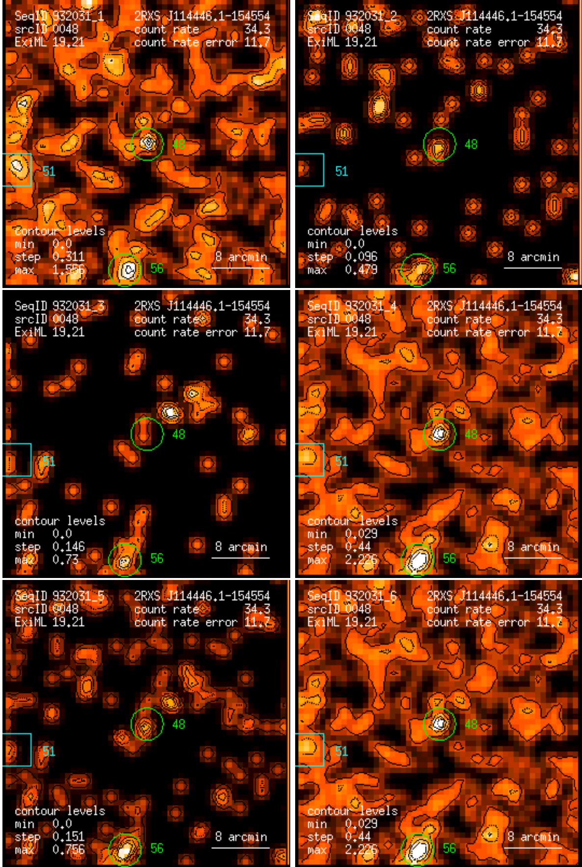
Figure 48: RASS 932031: detection 0048: band rate images, Gaussian filter: (1) PSPC channels 11 – 41, (2) 52 – 90, (3) 91 – 201, (4) 11 – 235, (5) 52 – 201, (6) 11 – 201. Broad band rates in counts/ks. Band rate contour levels in counts/ks/arcmin 2 .
