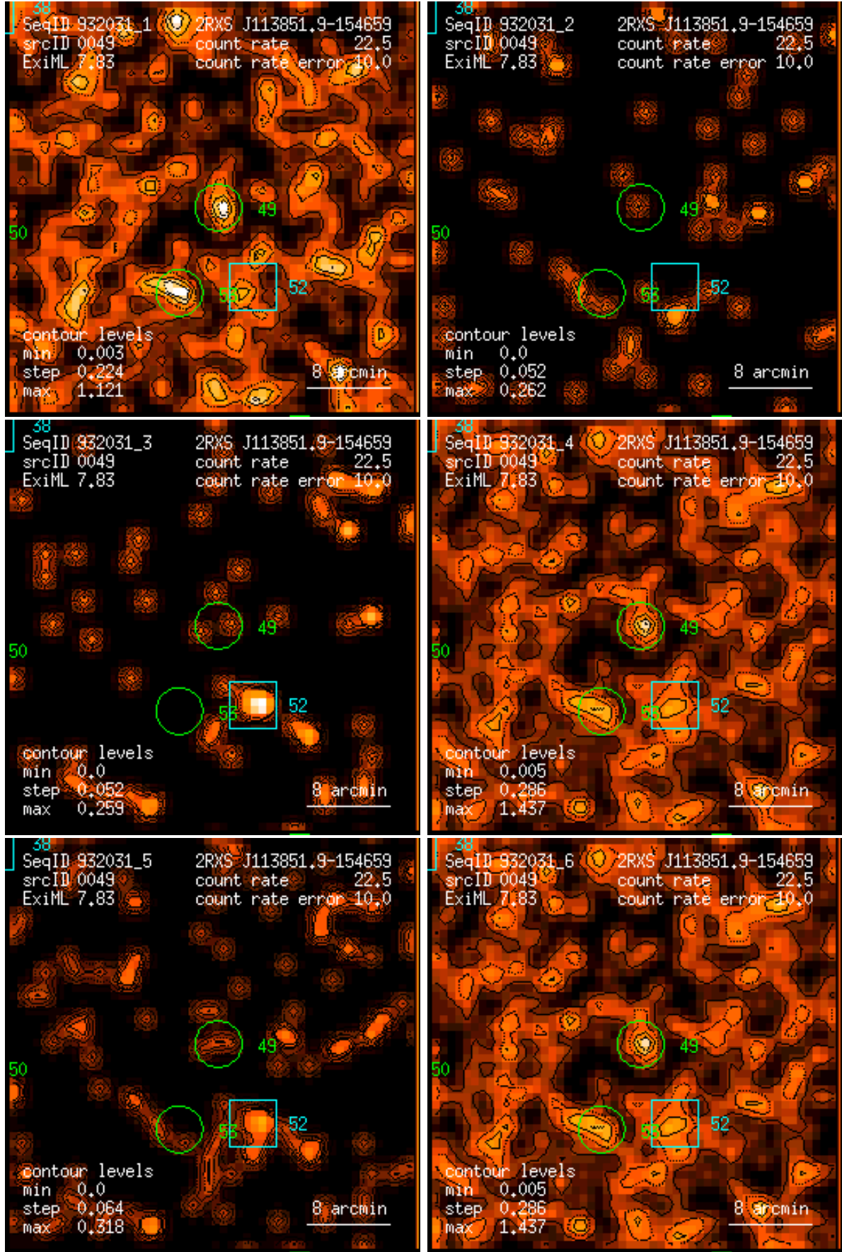
Figure 49: RASS 932031: detection 0049: band rate images, Gaussian filter: (1) PSPC channels 11 – 41, (2) 52 – 90, (3) 91 – 201, (4) 11 – 235, (5) 52 – 201, (6) 11 – 201. Broad band rates in counts/ks. Band rate contour levels in counts/ks/arcmin 2 .
