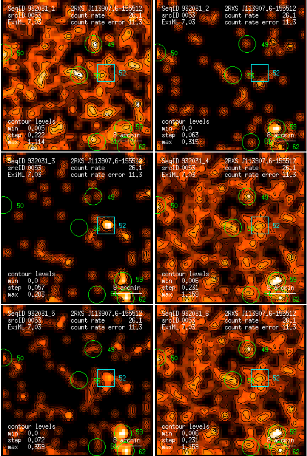
Figure 53: RASS 932031: detection 0053: band rate images, Gaussian filter: (1) PSPC channels 11 – 41, (2) 52 – 90, (3) 91 – 201, (4) 11 – 235, (5) 52 – 201, (6) 11 – 201. Broad band rates in counts/ks. Band rate contour levels in counts/ks/arcmin 2 .
