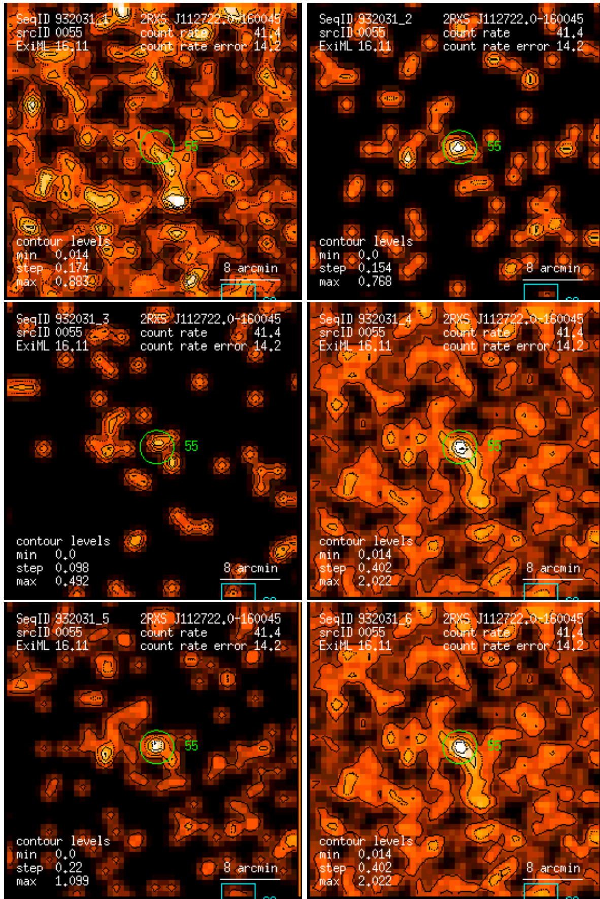
Figure 55: RASS 932031: detection 0055: band rate images, Gaussian filter: (1) PSPC channels 11 – 41, (2) 52 – 90, (3) 91 – 201, (4) 11 – 235, (5) 52 – 201, (6) 11 – 201. Broad band rates in counts/ks. Band rate contour levels in counts/ks/arcmin 2 .
