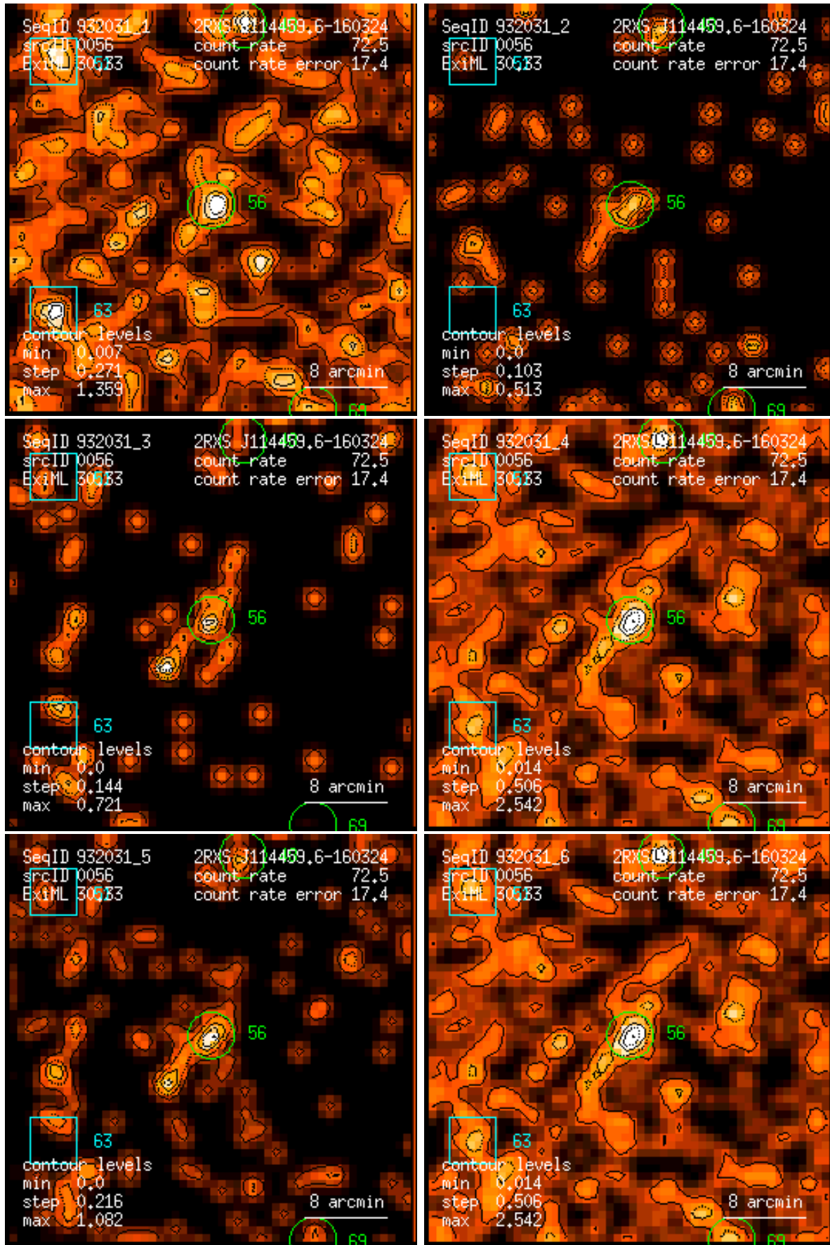
Figure 56: RASS 932031: detection 0056: band rate images, Gaussian filter: (1) PSPC channels 11 – 41, (2) 52 – 90, (3) 91 – 201, (4) 11 – 235, (5) 52 – 201, (6) 11 – 201. Broad band rates in counts/ks. Band rate contour levels in counts/ks/arcmin 2 .
