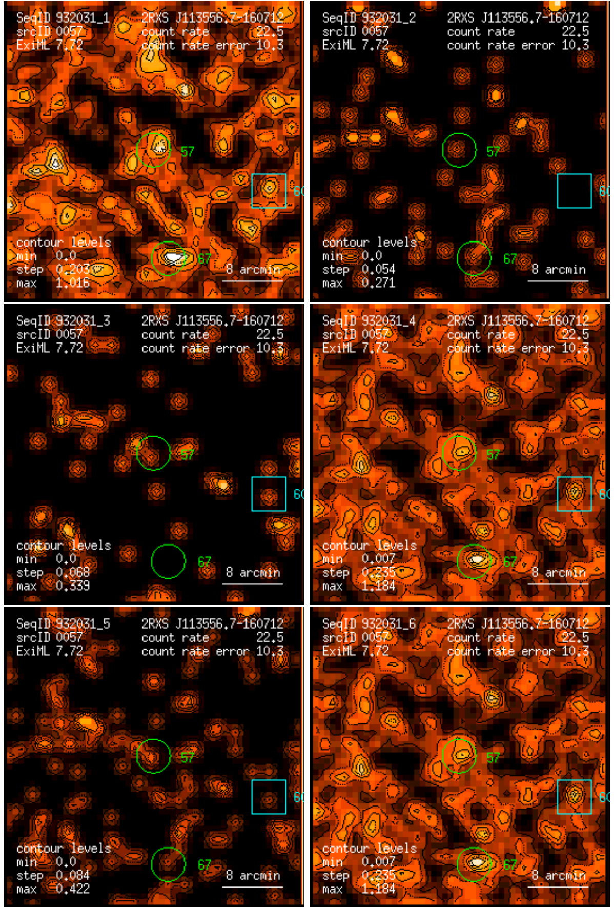
Figure 57: RASS 932031: detection 0057: band rate images, Gaussian filter: (1) PSPC channels 11 – 41, (2) 52 – 90, (3) 91 – 201, (4) 11 – 235, (5) 52 – 201, (6) 11 – 201. Broad band rates in counts/ks. Band rate contour levels in counts/ks/arcmin 2 .
