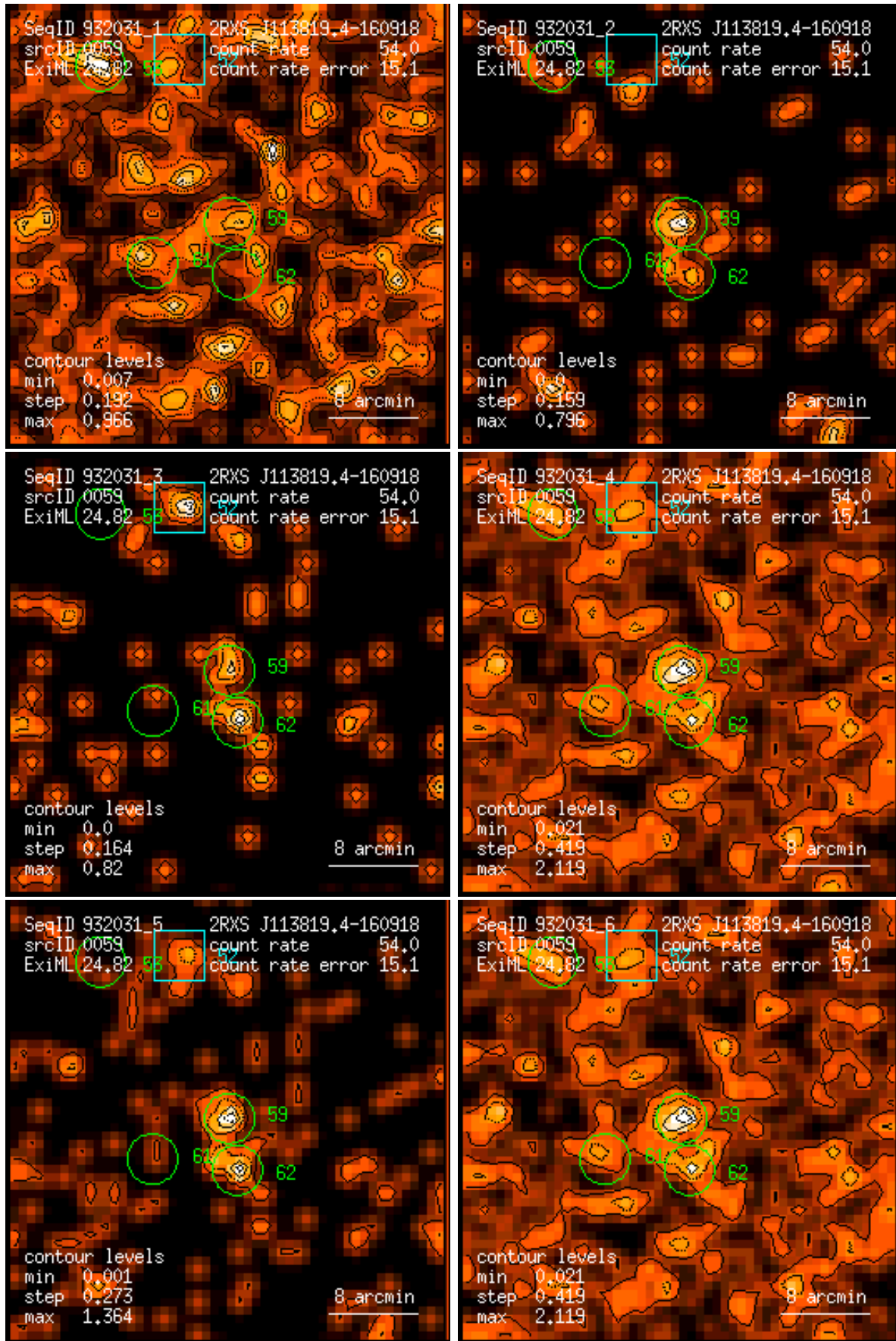
Figure 59: RASS 932031: detection 0059: band rate images, Gaussian filter: (1) PSPC channels 11 – 41, (2) 52 – 90, (3) 91 – 201, (4) 11 – 235, (5) 52 – 201, (6) 11 – 201. Broad band rates in counts/ks. Band rate contour levels in counts/ks/arcmin 2 .
