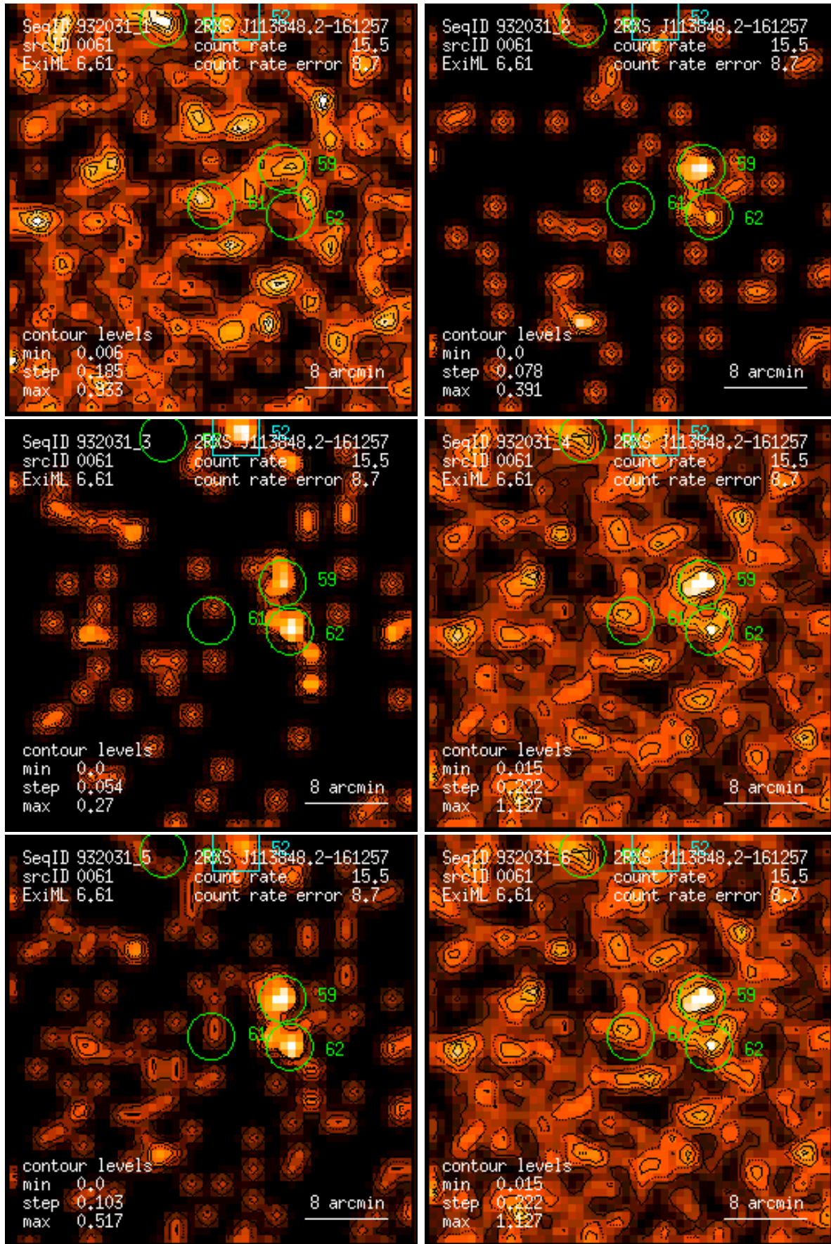
Figure 61: RASS 932031: detection 0061: band rate images, Gaussian filter: (1) PSPC channels 11 – 41, (2) 52 – 90, (3) 91 – 201, (4) 11 – 235, (5) 52 – 201, (6) 11 – 201. Broad band rates in counts/ks. Band rate contour levels in counts/ks/arcmin 2 .
