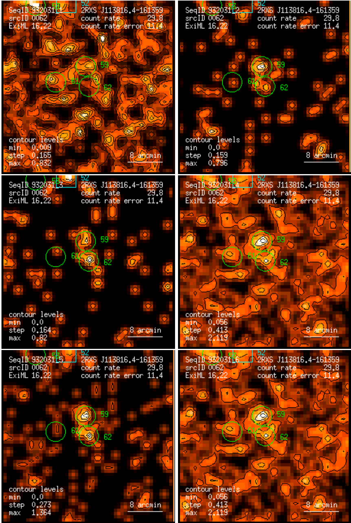
Figure 62: RASS 932031: detection 0062: band rate images, Gaussian filter: (1) PSPC channels 11 – 41, (2) 52 – 90, (3) 91 – 201, (4) 11 – 235, (5) 52 – 201, (6) 11 – 201. Broad band rates in counts/ks. Band rate contour levels in counts/ks/arcmin 2 .
