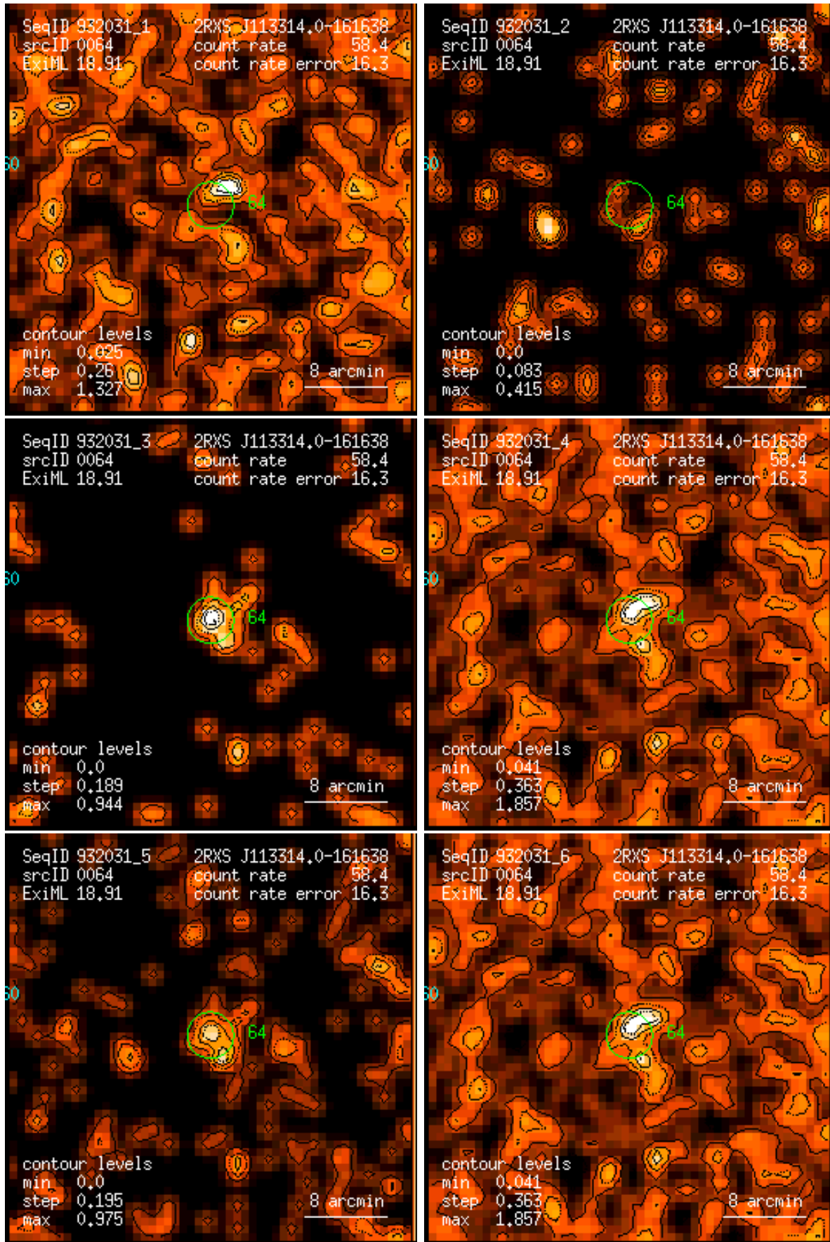
Figure 64: RASS 932031: detection 0064: band rate images, Gaussian filter: (1) PSPC channels 11 – 41, (2) 52 – 90, (3) 91 – 201, (4) 11 – 235, (5) 52 – 201, (6) 11 – 201. Broad band rates in counts/ks. Band rate contour levels in counts/ks/arcmin 2 .
