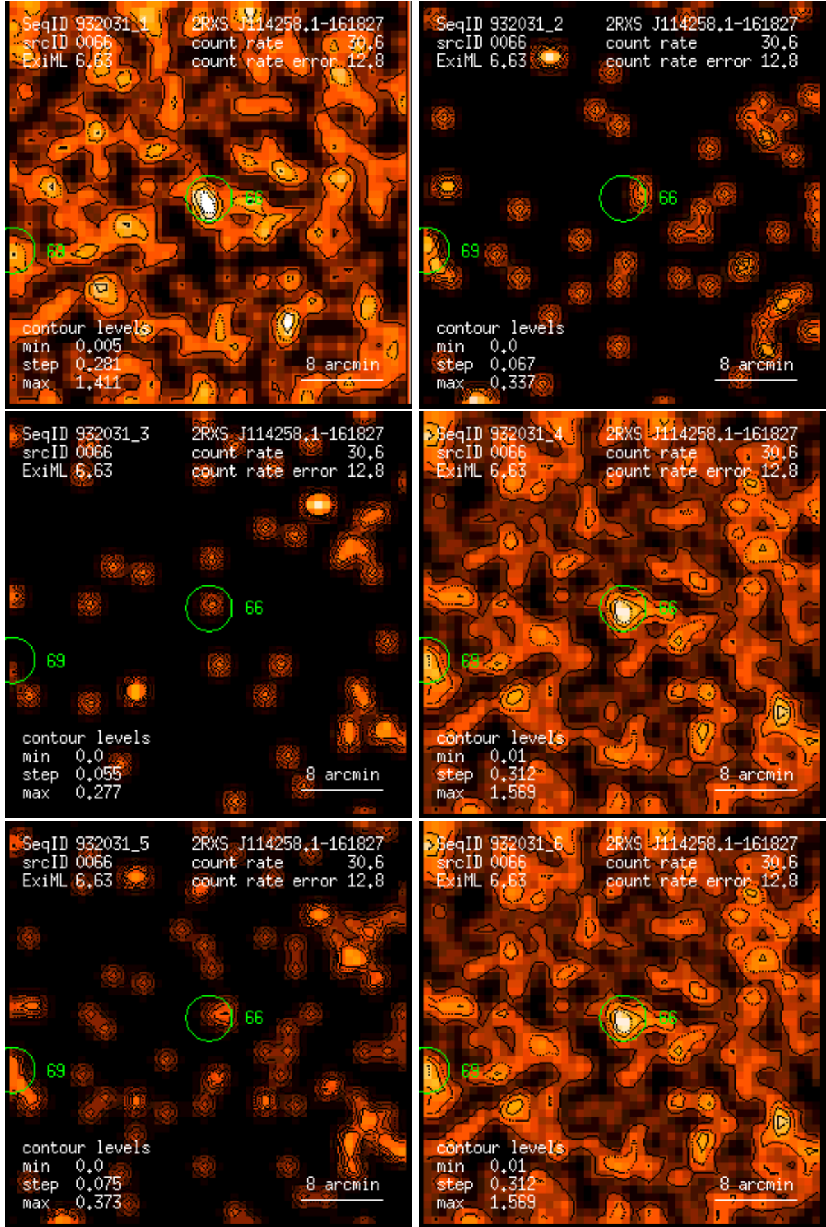
Figure 66: RASS 932031: detection 0066: band rate images, Gaussian filter: (1) PSPC channels 11 – 41, (2) 52 – 90, (3) 91 – 201, (4) 11 – 235, (5) 52 – 201, (6) 11 – 201. Broad band rates in counts/ks. Band rate contour levels in counts/ks/arcmin 2 .
