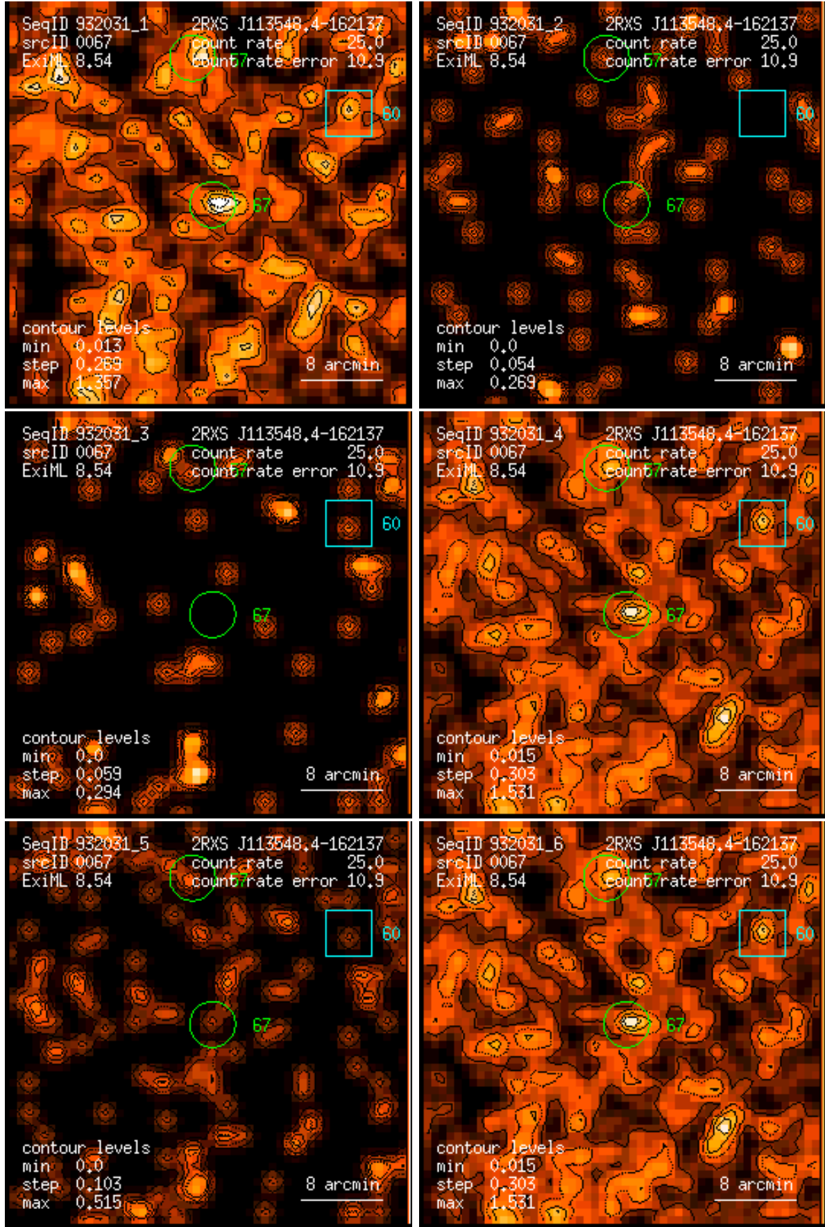
Figure 67: RASS 932031: detection 0067: band rate images, Gaussian filter: (1) PSPC channels 11 – 41, (2) 52 – 90, (3) 91 – 201, (4) 11 – 235, (5) 52 – 201, (6) 11 – 201. Broad band rates in counts/ks. Band rate contour levels in counts/ks/arcmin 2 .
