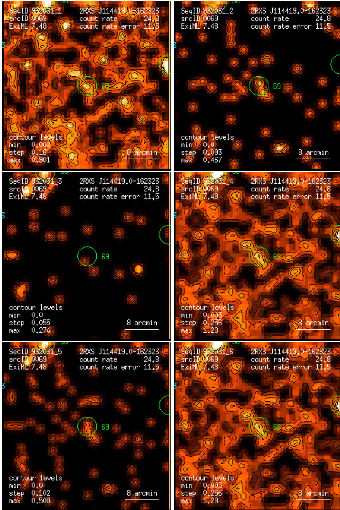
Figure 69: RASS 932031: detection 0069: band rate images, Gaussian filter: (1) PSPC channels 11 – 41, (2) 52 – 90, (3) 91 – 201, (4) 11 – 235, (5) 52 – 201, (6) 11 – 201. Broad band rates in counts/ks. Band rate contour levels in counts/ks/arcmin 2 .
