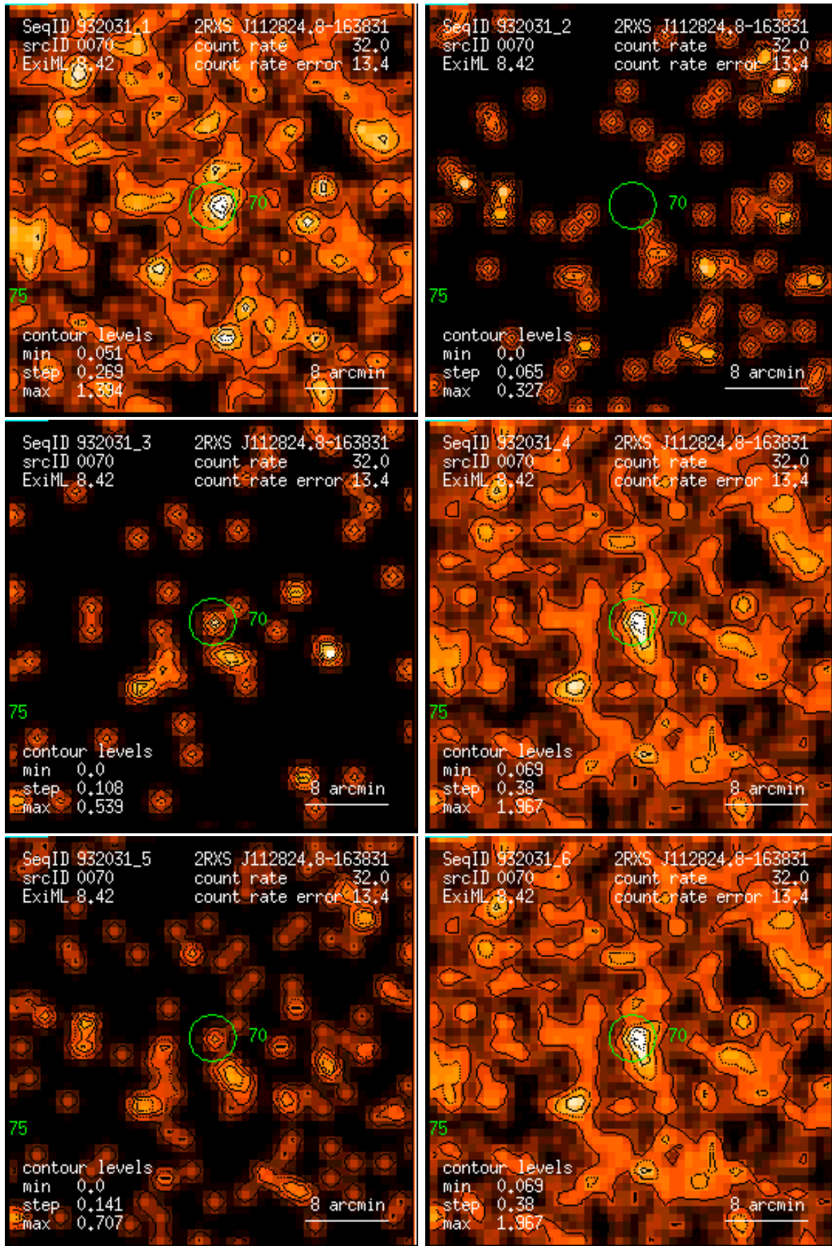
Figure 70: RASS 932031: detection 0070: band rate images, Gaussian filter: (1) PSPC channels 11 – 41, (2) 52 – 90, (3) 91 – 201, (4) 11 – 235, (5) 52 – 201, (6) 11 – 201. Broad band rates in counts/ks. Band rate contour levels in counts/ks/arcmin 2 .
