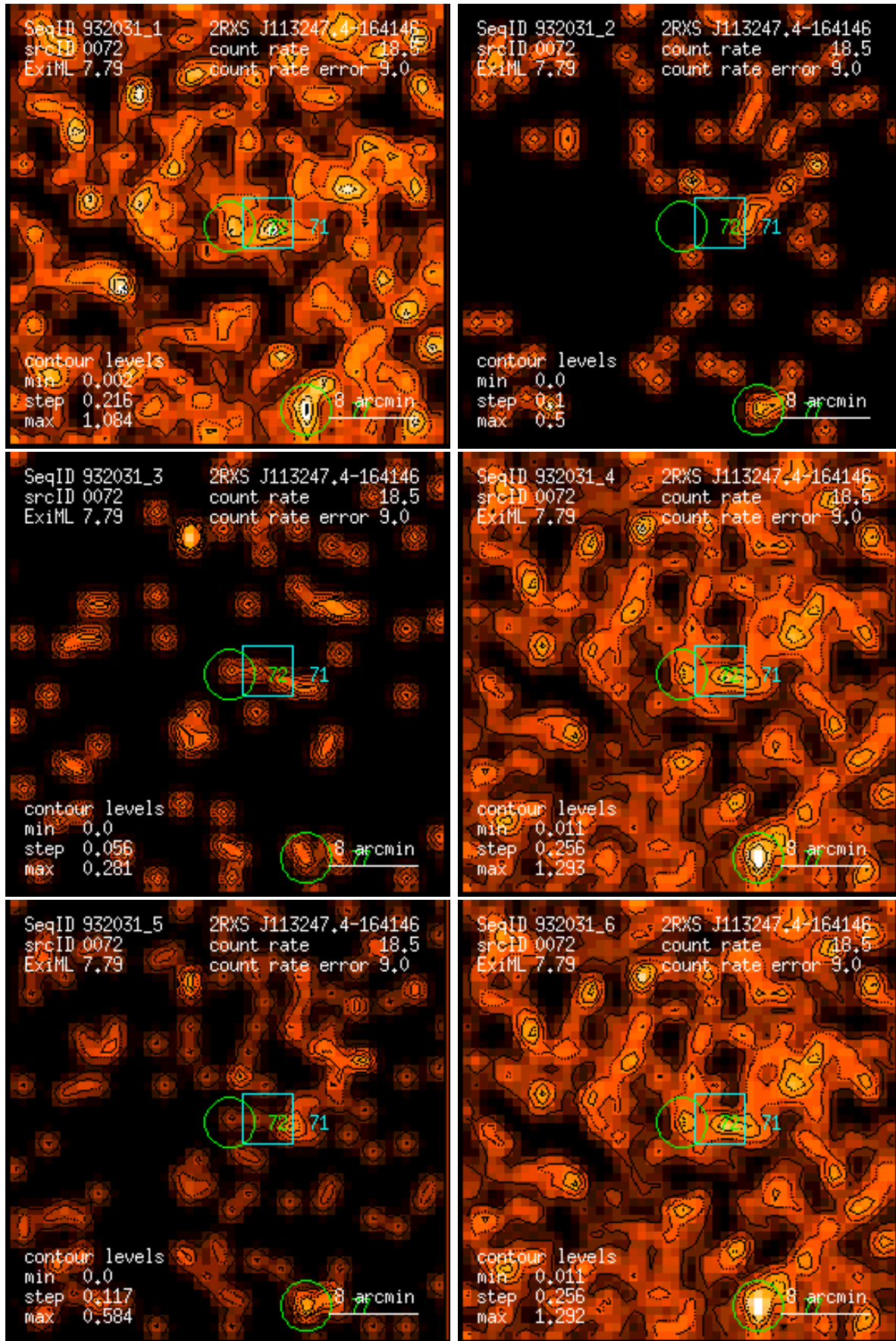
Figure 72: RASS 932031: detection 0072: band rate images, Gaussian filter: (1) PSPC channels 11 – 41, (2) 52 – 90, (3) 91 – 201, (4) 11 – 235, (5) 52 – 201, (6) 11 – 201. Broad band rates in counts/ks. Band rate contour levels in counts/ks/arcmin 2 .
