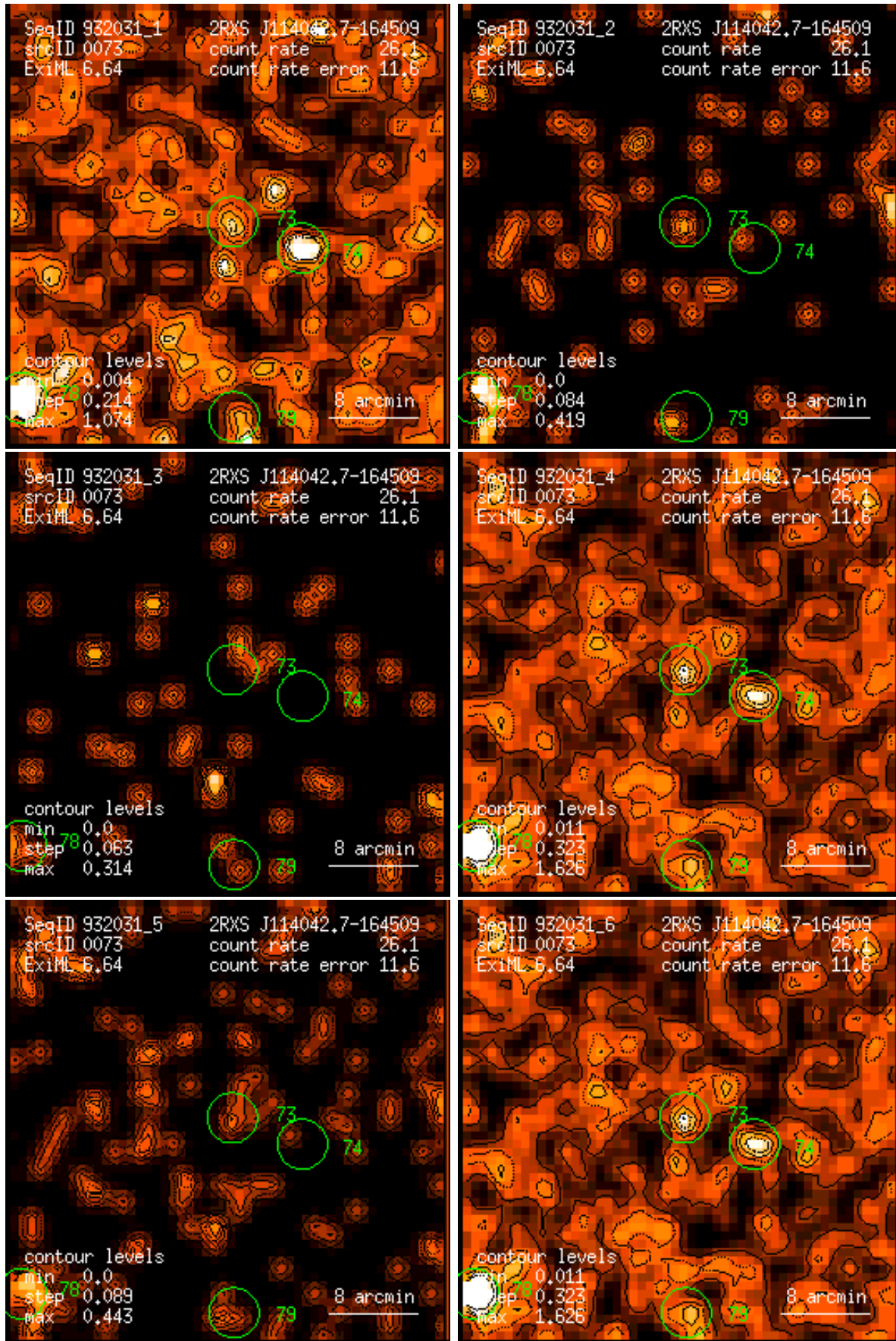
Figure 73: RASS 932031: detection 0073: band rate images, Gaussian filter: (1) PSPC channels 11 – 41, (2) 52 – 90, (3) 91 – 201, (4) 11 – 235, (5) 52 – 201, (6) 11 – 201. Broad band rates in counts/ks. Band rate contour levels in counts/ks/arcmin 2 .
