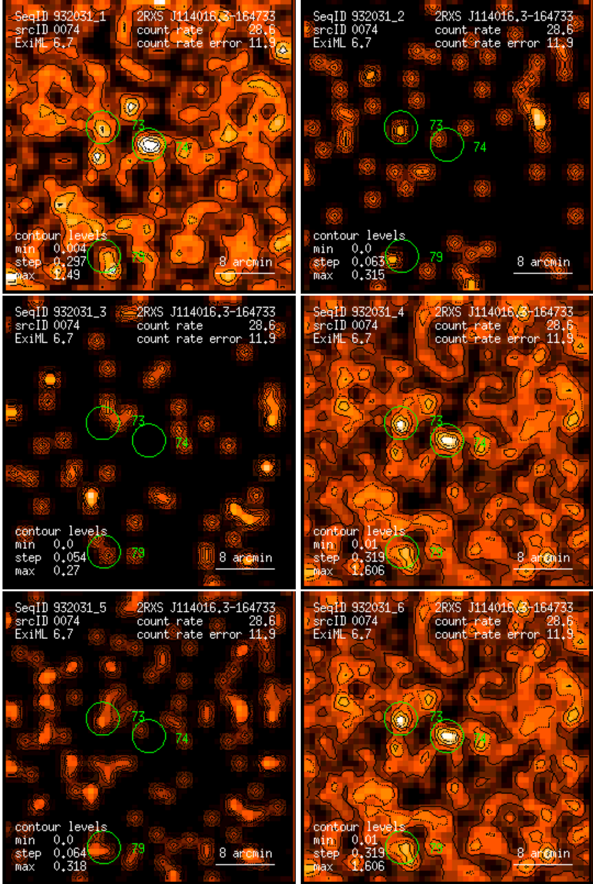
Figure 74: RASS 932031: detection 0074: band rate images, Gaussian filter: (1) PSPC channels 11 – 41, (2) 52 – 90, (3) 91 – 201, (4) 11 – 235, (5) 52 – 201, (6) 11 – 201. Broad band rates in counts/ks. Band rate contour levels in counts/ks/arcmin 2 .
