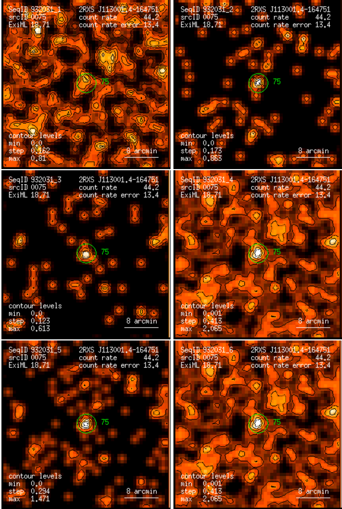
Figure 75: RASS 932031: detection 0075: band rate images, Gaussian filter: (1) PSPC channels 11 – 41, (2) 52 – 90, (3) 91 – 201, (4) 11 – 235, (5) 52 – 201, (6) 11 – 201. Broad band rates in counts/ks. Band rate contour levels in counts/ks/arcmin 2 .
