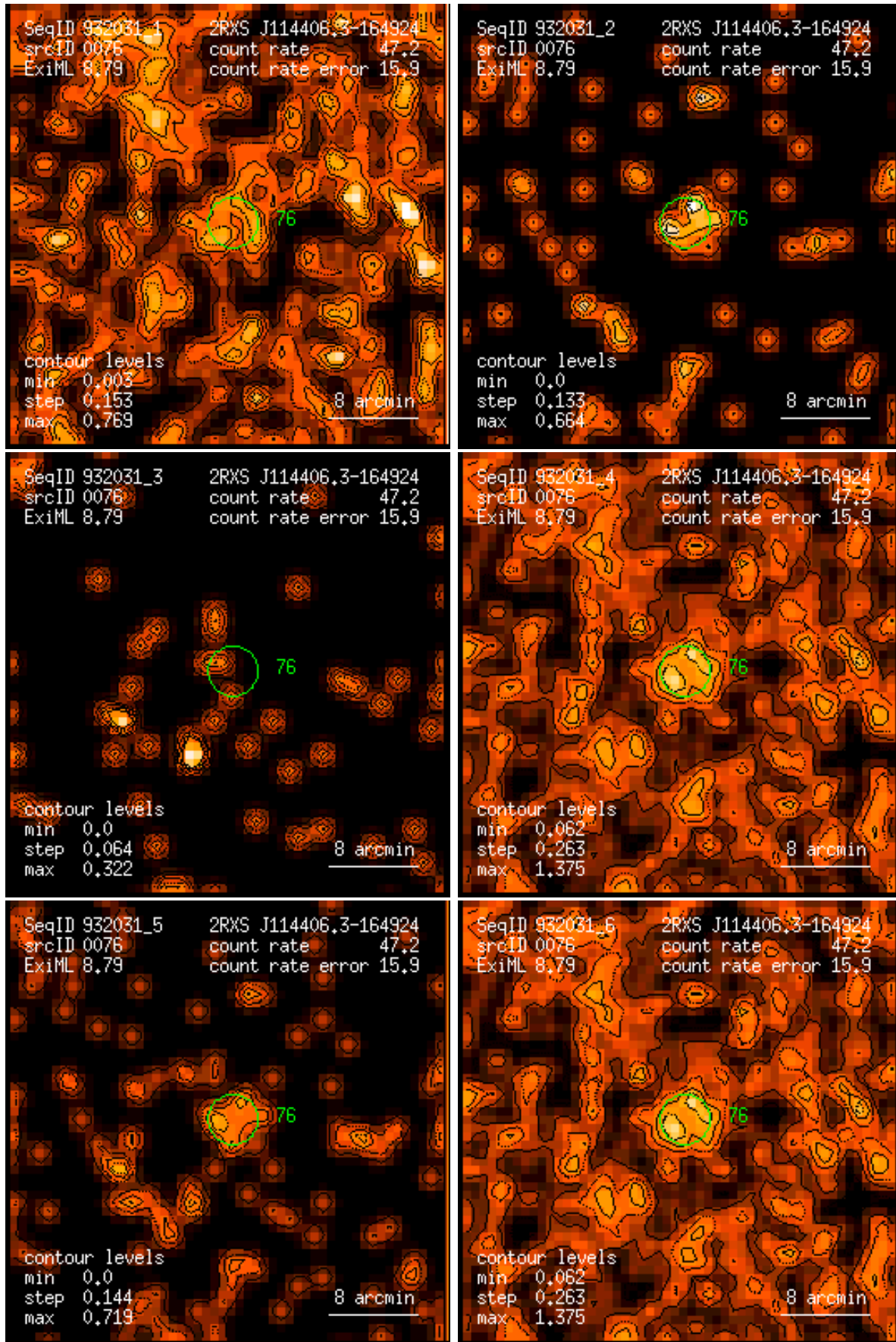
Figure 76: RASS 932031: detection 0076: band rate images, Gaussian filter: (1) PSPC channels 11 – 41, (2) 52 – 90, (3) 91 – 201, (4) 11 – 235, (5) 52 – 201, (6) 11 – 201. Broad band rates in counts/ks. Band rate contour levels in counts/ks/arcmin 2 .
